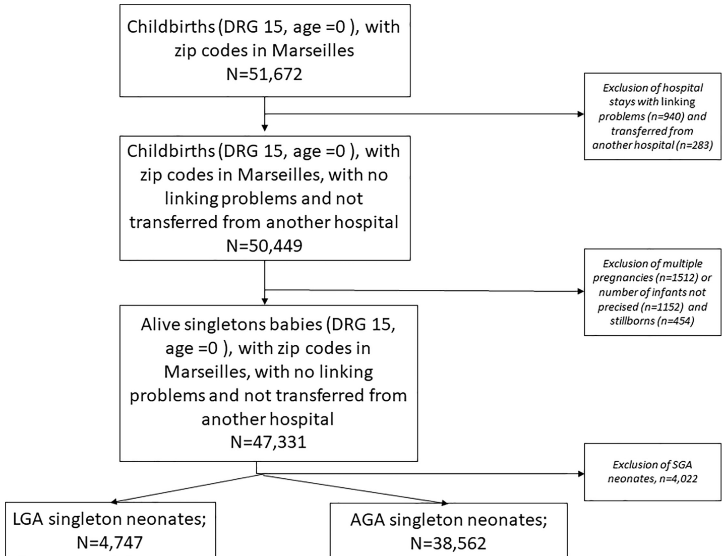
Fig 2. Flowchart.
