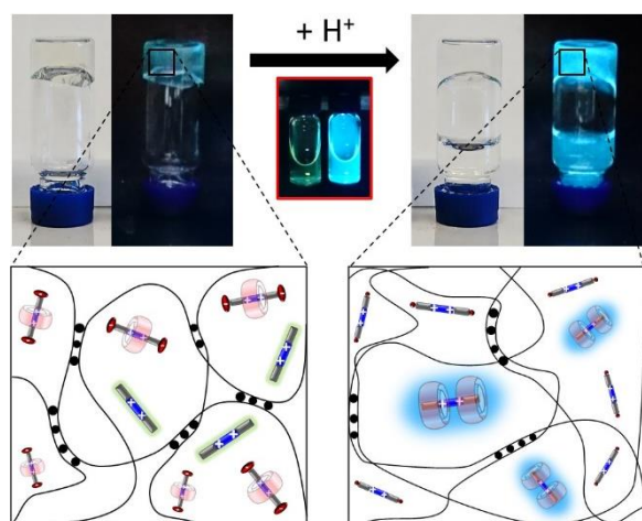
Figure 5. Hydrogels featuring the \text{PVP}^2\text{-CB[7]} kinetic trap and \text{DTV} showing weak emission (left) in basic conditions but strong fluorescence (right) after contact with an acidic solution as a result of \text{CB[7]} release and subsequent capture by \text{DTV} (red borders inset: identical solutions before (left) and after (right) acid addition without alginate and \text{CaCl}_2 ).
