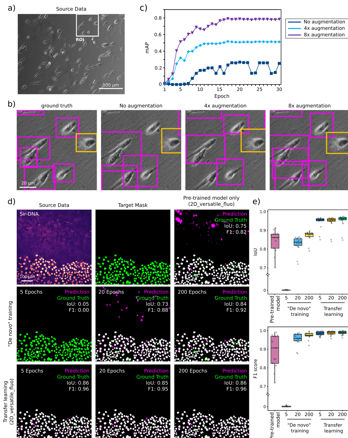
Fig. 9 Data augmentation and Transfer learning can improve performance. a–c Data augmentation can improve prediction performance. YOLOv2 cell shape detection applied to bright-field time-lapse dataset. a Raw bright-field input image. b Ground-truth and YOLOv2 model predictions (after 30 epochs) with increasing amounts of data augmentation. The original dataset contained 30 images which were first augmented by vertical and horizontal mirroring and then by 90° rotations. c mAP (mean average precision) as a function of epoch number for different levels of data augmentation. d, e These panels display an example of how transfer learning using a pretrained model can lead to very high-quality StarDist prediction even after only 5 epochs. This figure also highlights that using a pretrained model, even when trained on a large dataset, can lead to inappropriate results. d Examples of StarDist segmentation results obtained using models trained using 5, 20 or 200 epochs and using a blank model (“De novo” training) or the 2D-versatile-fluo as a starting point (transfer learning). e StarDist QC metrics obtained with the models highlighted in (d) (n = 13 images). The IoU (intersection over union) scores are calculated over the whole image, while the F1 scores are calculated on a per-object basis. Results are displayed as boxplots which represent the median and the 25th and 75th percentiles (interquartile range); outliers are represented by dots 96 . Note that the axes of both graphs are cut. Source data for panel (c) and (e) are provided in the Source Data file.
