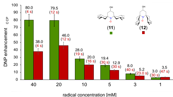
Figure 2: ^1\text{H} MAS-DNP enhancements measured via ^1\text{H} - ^{13}\text{C} CP for the mono-radicals O-MbPyTol ( (11) in green) and C-MbPyTol ( (12) in red) in \text{DMSO-}d_6\text{:D}_2\text{O:H}_2\text{O} (60:30:10 v/v/v) at different radical concentrations at 9.4 T and 100 K. The observed \epsilon_{C\ CP} value is indicated in black above the bar. The build-up time of the solvent ^1\text{H} signals is given in parentheses. A 10% confidence interval on the measured enhancement is indicated.
