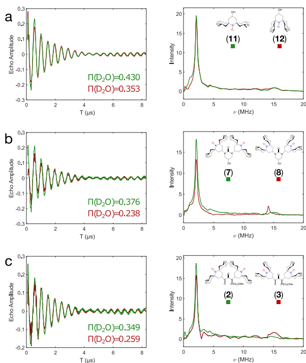
Figure 5: Three-pulse ESEEM time-domain data and the corresponding magnitude spectra in (a) for (11) and (12) in \text{DMSO-}d_6\text{:D}_2\text{O:H}_2\text{O} (60:30:10 v/v/v); in (b) for (7) and (8) in \text{DMSO-}d_6\text{:D}_2\text{O:H}_2\text{O} (60:30:10 v/v/v); in (c) for (2) and (3) in \text{glycerol-}d_8\text{:D}_2\text{O:H}_2\text{O} (60:30:10 v/v/v) at 50 K and 200 \mu\text{M} . The solvent accessibility parameter \Pi(\text{D}_2\text{O}) , defined in eq. SI-6, is always larger for the O- class: \Pi^{\text{O}}(\text{D}_2\text{O}) > \Pi^{\text{C}}(\text{D}_2\text{O}) . We note that in the case of C-MPyPolC 6 OH (8) the proton modulation is not completely suppressed leading to a small peak at the ^1\text{H} Larmor frequency at circa 15 MHz.
