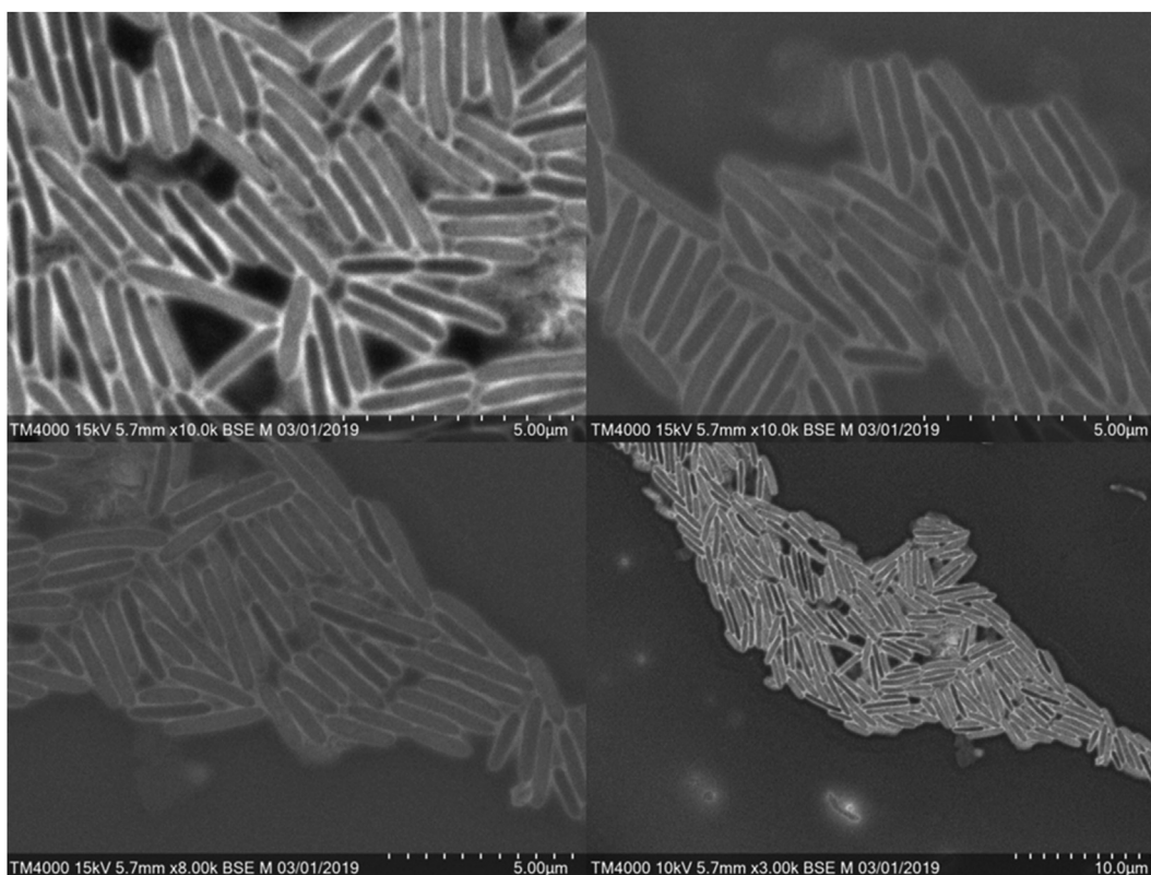
FIG. 2. Scanning electron microscopy (SEM) of stained Luxibacter massiliensis gen. nov., sp. nov. A colony was collected from agar and immersed into a 2.5% glutaraldehyde fixative solution. Then a drop of suspension was directly deposited on a poly-L-lysine-coated microscope slide for 5 minutes and treated with 1% phosphotungstic acid (PTA) aqueous solution (pH 2.0) for 2 minutes to increase SEM image contrast. The slide was gently washed in water, air dried and examined with a Hitachi TM4000Plus tabletop microscope (Hitachi High-Tech, Tokyo, Japan). Scales and acquisition settings are shown.
