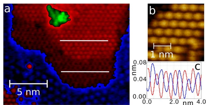
Figure 3 | Two different contrasts originating from a double tip with two different chemical apices observed upon imaging the second silicene layer. (a) STM topography image (filled states, U_{\text{bias}} = -0.4 V, I = 0.1 nA). (b) The second layer of silicene, nc-AFM topography image ( \Delta f = -4.1 Hz, A_{\text{p-p}} = 7.5 nm), (c) Line profiles red/blue corresponding to the two upper/lower white lines in image (a).
