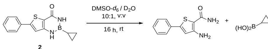
Scheme 3. Observed degradation of 2 under neutral aqueous conditions.
