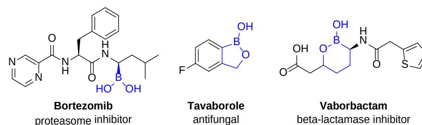
Figure 2. Examples of marketed boron-containing drugs.
