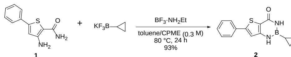
Scheme 2. Synthesis of compound 2 .
