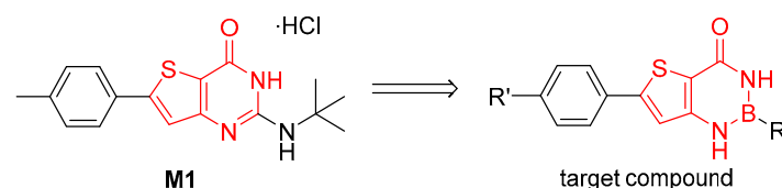
Scheme 1. Scaffold hopping strategy for compound M1.
