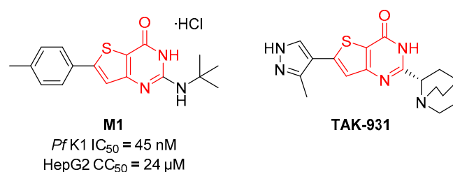
Figure 1. Chemical structures of compounds M1 and TAK-931.
