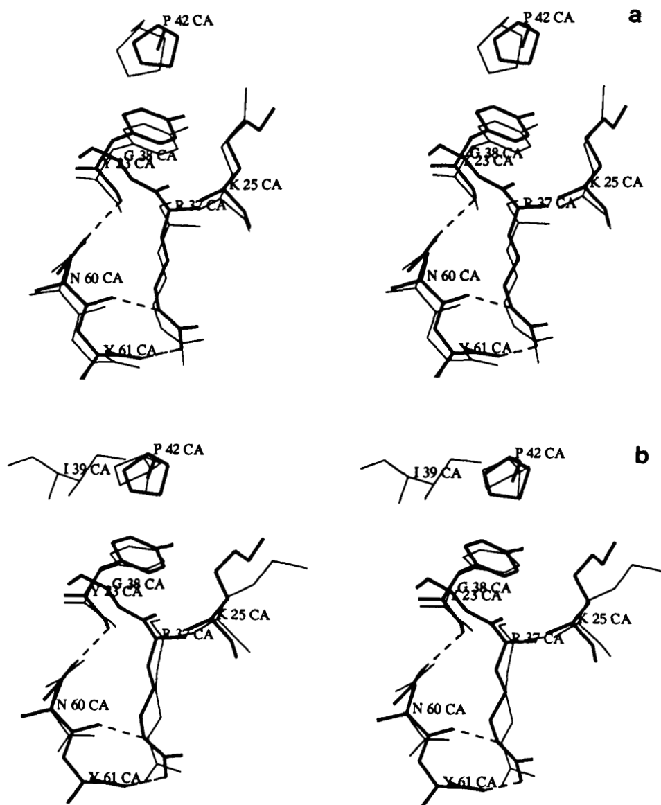
FIG. 8. Stereo drawing of the environment around Tyr 23 . Comparison of (a) fasciculin 1 (thick line) and erabutoxin b and (b) fasciculin 1 and cardiotoxin V 4 1 . The superposition was done as described in the legend to Fig. 6. In b, the side chain of Tyr 61 has been omitted for clarity.
