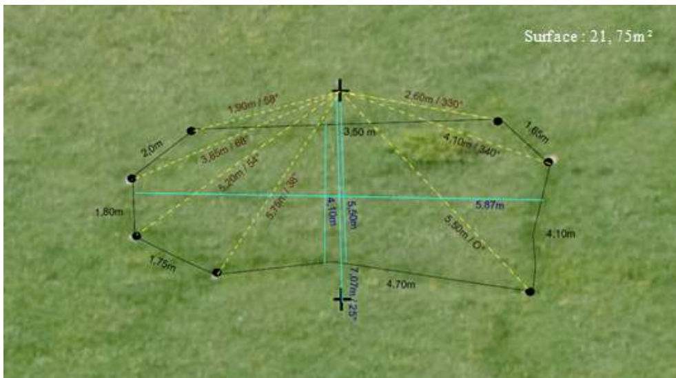
Figure 3: Morphotopographic parameters recorded on the three polygonal grounds, Dévoluy, Col du Noyer
