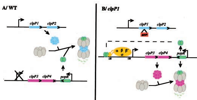
Fig. 7. Model of regulation of clpP3 operon. A. PopR degradation by ClpP1 and ClpP2 proteins forming a proteolytic complex in a wild-type strain.
