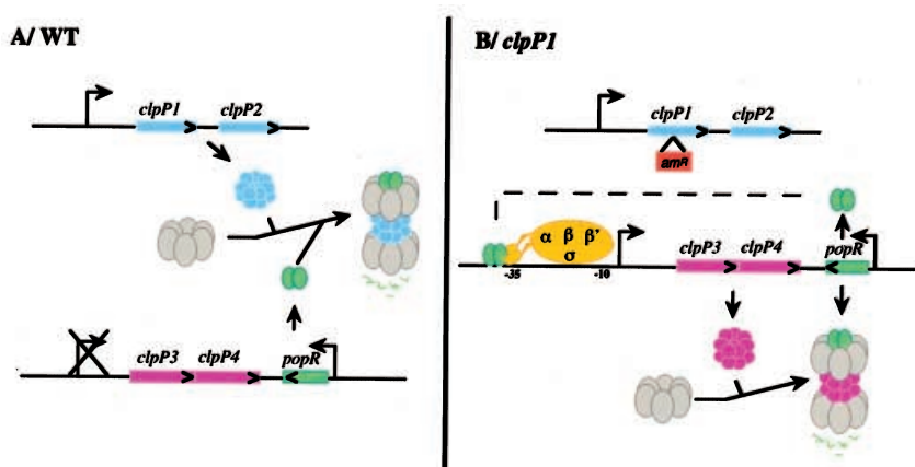
Fig. 7. Model of regulation of clpP3 operon. A. PopR degradation by ClpP1 and ClpP2 proteins forming a proteolytic complex in a wild-type strain. B. Stabilization of PopR and activation of clpP3 and clpP4 in the clpP1 mutant strain.
