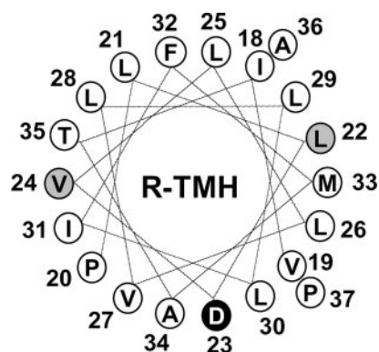
FIGURE 2. Summary of TolR cysteine substitutions phenotypes. The TolR anchor residues are represented on a helical wheel projection. The color code corresponds to the phenotype, as classified in Ref. 14. White , functional cysteine mutants (class I); black , nonfunctional mutants (class II); affected in TolQR complex assembly ; gray , discriminative mutants (class III, nonfunctional for the PMF-dependent outer membrane integrity, functional for the PMF-independent colicin import).
