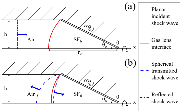
Fig. 3 Sketch of the gas lens configuration with the geometrical parameters : (a) before shock-interface interaction (b) after interaction.
