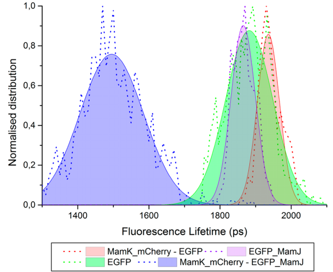
Figure 5. Distribution of the fluorescence lifetime values (dotted lines) fitted to a Gaussian function (filled area delimited by a line) of the E. coli strains expressing eGFP (green); eGFP_MamJ (purple); MamK_mCherry and eGFP (red); and MamK_mCherry and eGFP_MamJ (blue).
