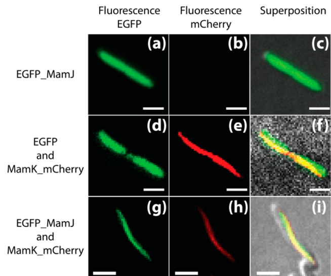
Figure 2. Fluorescence images of E. coli expressing: eGFP_MamJ (a, b, c), MamK_mCherry and eGFP (d, e, f), and MamK_mCherry and eGFP_MamJ (g, h, i). Excitation and emission wavelength of eGFP, i.e., 488 and 500–550 nm (a, d, g); excitation and emission wavelength of mCherry, i.e., 561 and 570–640 nm (b, e, h). Superposition of images (a) and (b) on a transmission image (c); (d) and (e) on a transmission image (f); and (g) and (h) on a transmission image (i). Scale bar 2 \mu m.
