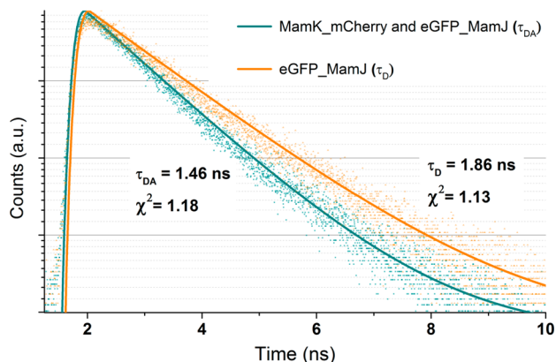
Figure 3. Fluorescence lifetime decay curves of eGFP in E. coli expressing MamK_mCherry and eGFP_MamJ (blue points, bottom) and in E. coli expressing eGFP_MamJ (orange points, top). Single-exponential function best fitting the data points (lines).
