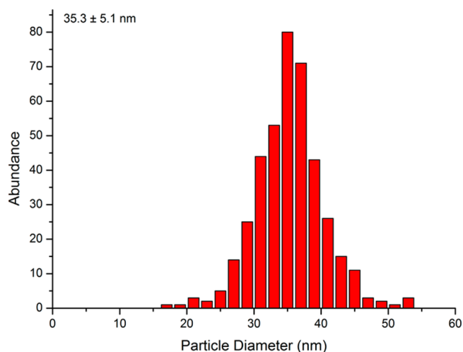
Figure 3. Particle size distribution of magnetite particles formed in the presence of polyR.
