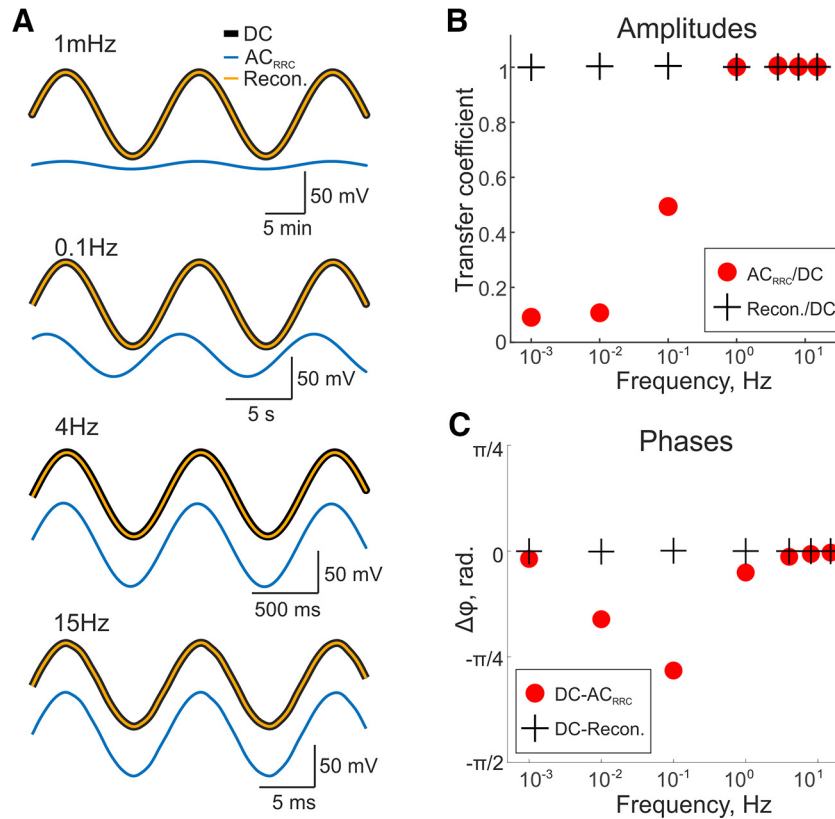
Figure 2. Investigation of the RRC filter characteristics using test sine signals. A , Examples of sine signals at frequencies 1 mHz, 0.1 Hz, 4 Hz, and 15 Hz recorded simultaneously by the AC RRC (blue trace) and DC (black trace) channels as well as the result of signal reconstruction via IF EMPIR (inverse filter empirical) from AC RRC recording (orange trace). B , Amplitude ratio of sine signal recorded in AC RRC and DC modes at seven selected frequencies: 1 mHz, 10 mHz, 0.1 Hz, 1 Hz, 4 Hz, 8 Hz, and 15 Hz (red circles) and the amplitude ratio of reconstructed signal relative to the original signal recorded in DC mode (black crosses). C , Phase difference between DC and AC RRC signals (red circles) containing sine signals at the same frequencies as shown in panel B , and the phase difference between DC and reconstructed from AC RRC signals (black crosses).
