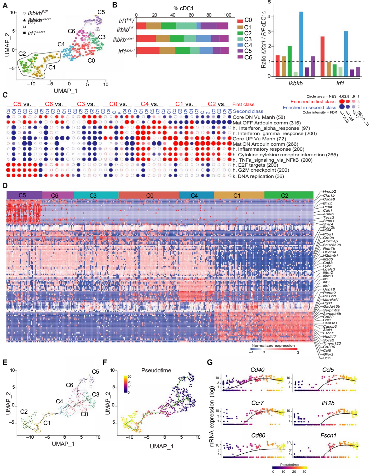
Fig. 6. IKK \beta and IRF1 coordinate intratumoral cDC1 maturation. (A) UMAP and graph-based cell clustering for 360 bona fide cDC1s isolated from YUMM1.7 tumors of 16 female Ikkkb F/F , Ikkkb \Delta Xcr1 , Irf1 F/F , and Irf1 \Delta Xcr1 mice grown to a volume of 200 to 350 mm 3 ; seven distinct clusters are indicated C0 to C6. (B) Distribution of clusters among total cDC1s in each group (left) and proportions of individual cDC1 clusters in Ikkkb \Delta Xcr1 and Irf1 \Delta Xcr1 mice relative to their respective littermate controls ( Ikkkb F/F and Irf1 F/F ) (right). (C) BubbleMap showing the results of GSEA using hallmark, KEGG pathway, and published DC maturation gene sets performed with BubbleGUM for pairwise comparisons between clusters C0 to C6 shown in (A), as described in Fig. 2B. (D) Heatmap showing expression levels of selected genes across C0 to C6. (E and F) Single-cell trajectory inference by Monocle with projection onto the UMAP space, (E) showing Seurat clusters and (F) the pseudotime analysis using C5 as the root. (G) Expression pattern along Monocle pseudotime of selected genes related to cDC1.
