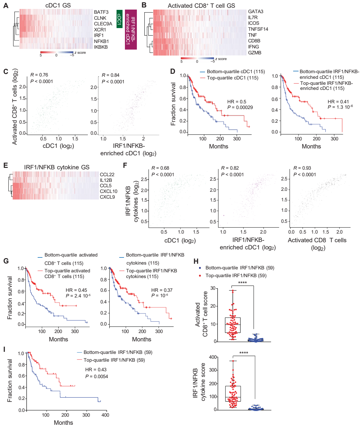
Fig. 7. NF- \kappa B/IRF1-enriched cDC1 GSs correlate with increased survival in patients with melanoma. (A) Heatmap showing the gene similarity-ordered, z-transformed expression values for cDC1 and NFKB/IRF1-enriched cDC1 GSs and (B) activated CD8 + T cell GS in patients with melanoma from TCGA datasets. CLNK, cytokine-dependent hematopoietic cell linker. CLEC9A (C-type lectin domain containing 9A), CLNK (cytokine dependent hematopoietic cell linker). (C) Spearman correlation between cDC1 GS or NFKB/IRF1-enriched cDC1 GS with activated CD8 + T cell GS in melanoma TCGA datasets. (D) Kaplan-Meier overall survival curves of TCGA patients with melanoma comparing top and bottom quartiles of cDC1 GS or NFKB/IRF1-enriched cDC1 GS. Hazard ratio (HR) and P value from univariate Cox regression are indicated. (E) Heatmap showing the gene similarity-ordered, z-transformed expression values for NFKB/IRF1-dependent chemokine GS in melanoma TCGA datasets. (F) Spearman correlation between cDC1 GS, NFKB/IRF1-enriched cDC1 GS, and activated CD8 + T cell GS with NFKB/IRF1-dependent chemokine GS in melanoma TCGA datasets. (G) Kaplan-Meier overall survival curves of TCGA patients with melanoma comparing top and bottom quartiles of activated CD8 + T cell GS or NFKB/IRF1-dependent chemokine GS. (H) Box plots comparing activated CD8 + T cell GS and NFKB/IRF1-dependent chemokine GS in top and bottom quartiles of NFKB/IRF1 expression in TCGA patients with melanoma bearing high cDC1 GS (top 50%). (I) Kaplan-Meier overall survival curve comparing top and bottom quartiles of NFKB/IRF1 expression in TCGA patients with melanoma bearing high cDC1 GS score (top 50%).
