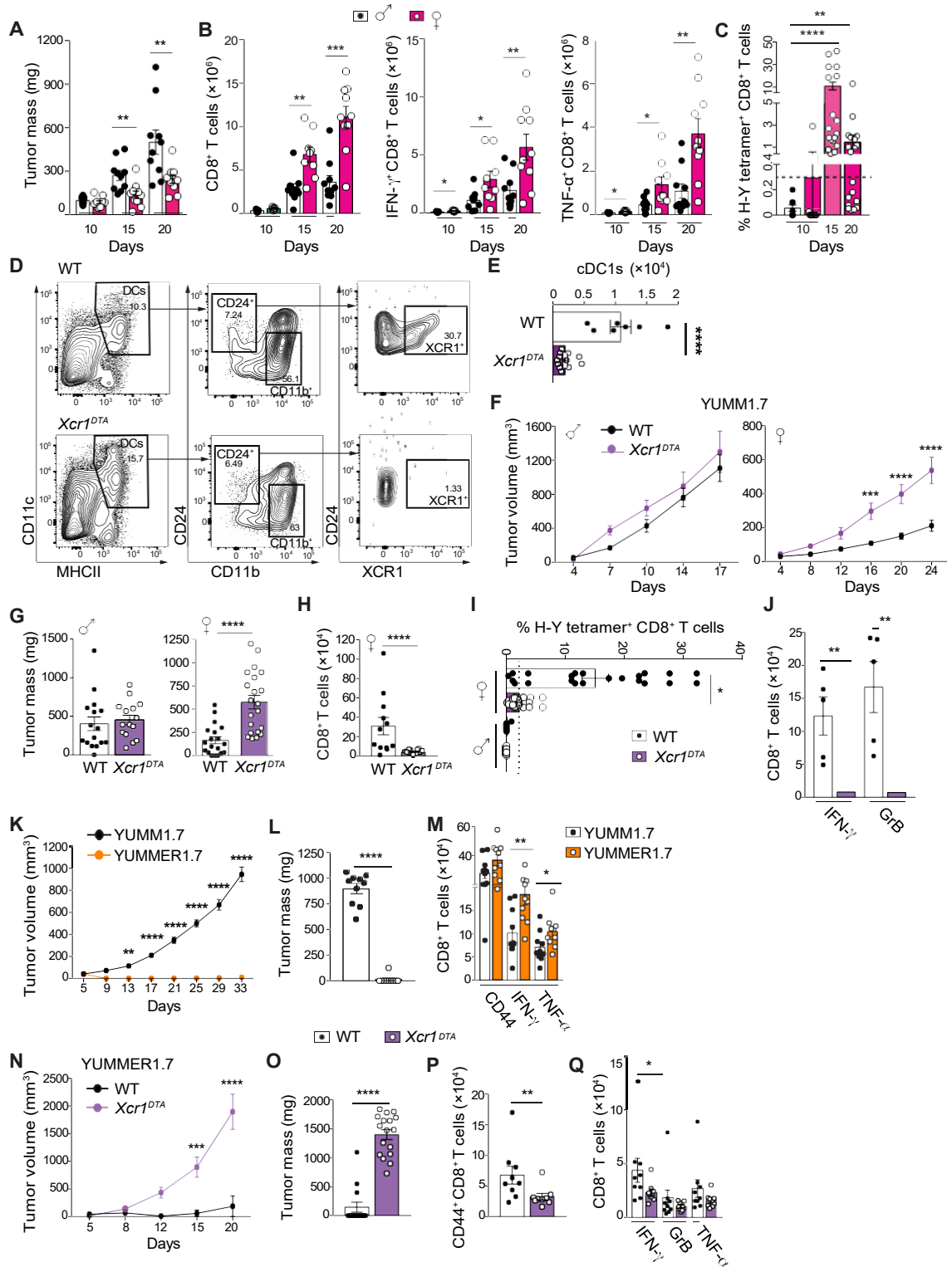
Fig. 1. cDC1s are required for control of immunogenic tumor growth. (A) YUMM1.7 tumor growth in male and female mice. (B) Quantification of tumor-infiltrating CD8 + T cells, and IFN- \gamma , or TNF- \alpha -producing CD8 + T cells, by flow cytometry in YUMM1.7 tumors from male and female mice at end point. (C) Tetramer analysis of H-Y-specific CD8 + T cells (Smcy (738–746) /H-2D b and Uty (243–254) /H-2D b ) in YUMM1.7 tumors.
