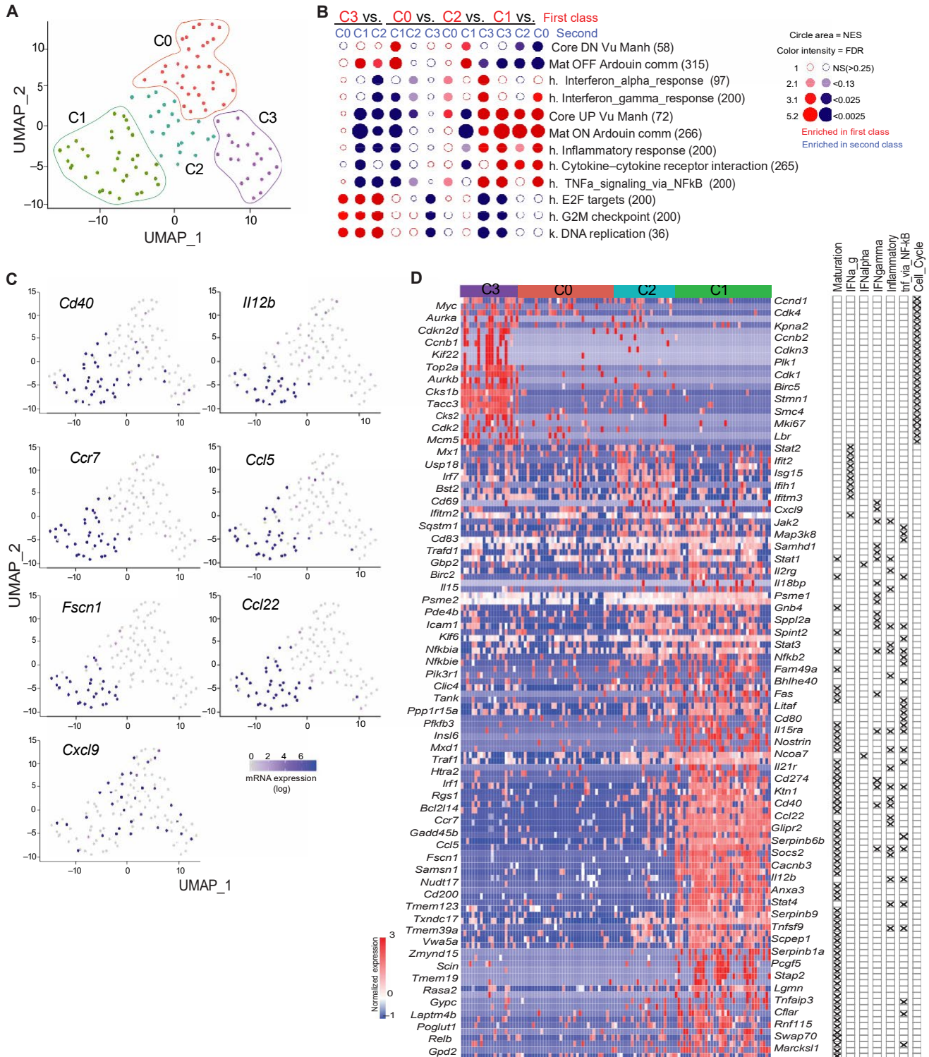
Fig. 2. Single-cell transcriptional profiling of cDC1s from immunogenic tumors. (A) Dimensionality reduction performed using the UMAP algorithm and graph-based cell clustering using Seurat, for 113 bona fide cDC1s sorted from YUMM1.7 tumors of eight female mice 10 days after engraftment. (B) BubbleMap showing results of GSEA with hallmark (h), KEGG pathway (k), and published DC maturation gene sets, performed by using BubbleGUM on pairwise comparisons between the clusters C0 to C3 shown in (A). Circle area indicates NES and color intensity the FDR. FDR was further corrected for multiple testing, leading to a higher stringency of the significance threshold. Core_DN_Vu_Manh and Core_UP_Vu_Manh correspond to gene sets down- or up-regulated, respectively, across human and mouse DC subsets during maturation in response to microbial stimuli (29). Mat_ON_Arduin_comm and Mat_OFF_Arduin_comm correspond to gene sets up- or down-regulated, respectively, during steady-state maturation of mouse cDC1s (31). Numbers in parentheses correspond to the number of genes. NS, not significant. (C) Expression levels of selected genes related to DC maturation, projected onto the UMAP space. (D) Heatmap showing expression of selected genes across C0 to C3 and association of individual genes to gene sets used in (B) (right).
