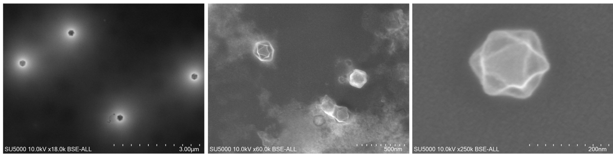
FIGURE 1 | Scanning electron microscopy of marseillevirus T19 particles. Micrographs of viral particles from culture supernatant. Technical settings and scale bars are indicated in the images.
