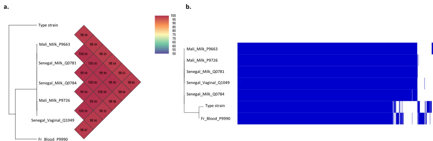
Fig 2. Endemic clonal circulation of L. monocytogenes in West Africa. (a) Genomic similarity estimated using Orthologous Average Nucleotide Identity Tool (OAT) software. (b) Pangenome carried out using the ROARY software.
