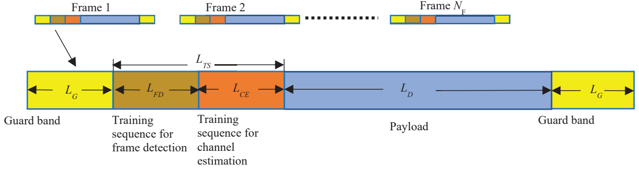
Fig. 2. Frame structure.
