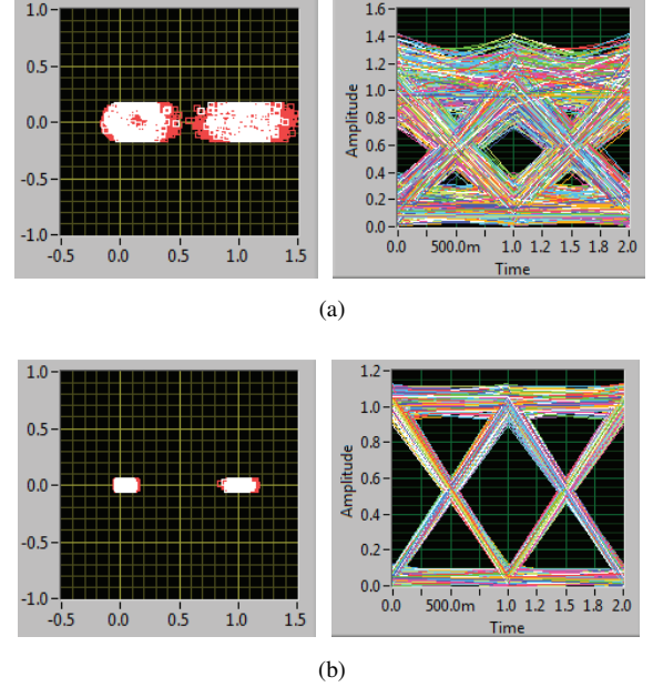
Fig. 5. Constellation and eye diagram of received signal at 1 meter in LOS scenario with strict alignment (a) without lens (b) with lens.
