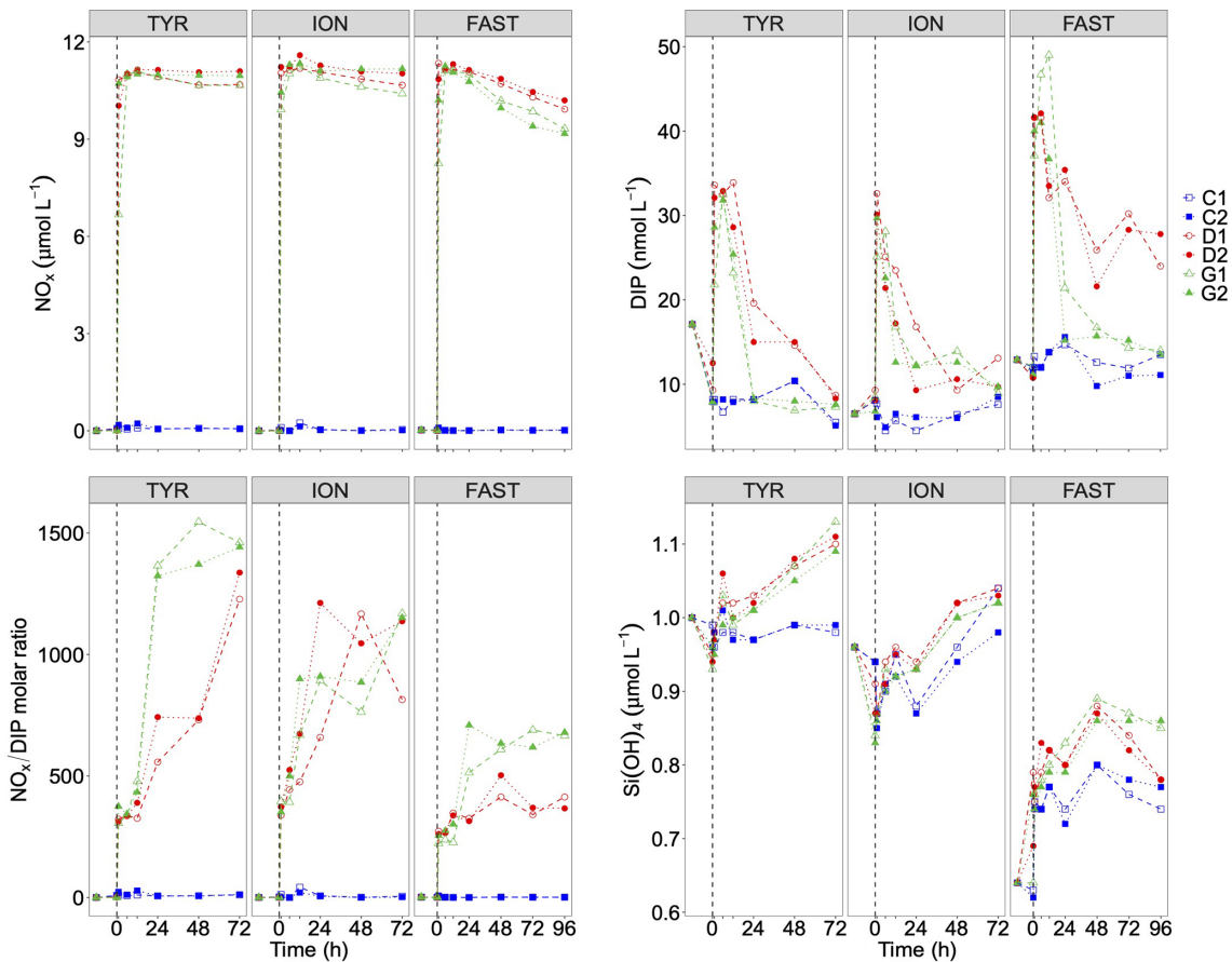
Figure 6. Nutrients (nitrate + nitrite): NO x , dissolved inorganic phosphorus: DIP, silicate: Si(OH) 4 and the molar ratio between NO x and DIP, measured in each tank during the experiments at TYR, ION and FAST. The dashed vertical line indicates the time of seeding (after t0).
