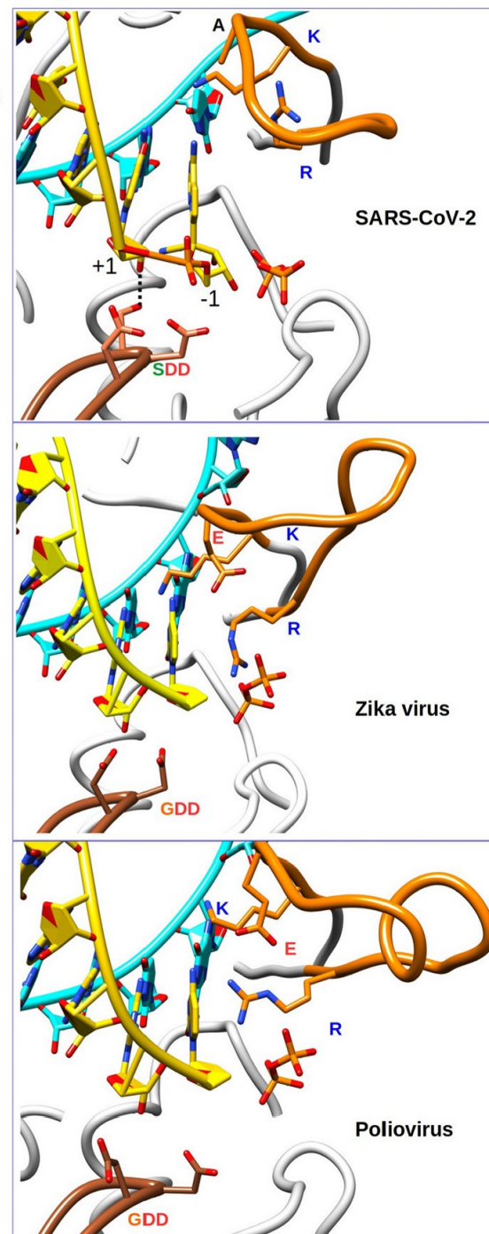
Figure 2. Sequences and structural features comparison of (+)RNA virus RNA-dependent RNA polymerase (RdRp) active sites order by genome size.
