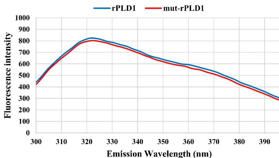
Figure 3. Intrinsic fluorescence emission of rPLD1 and mut-rPLD1. As seen here, both proteins have the similar fluorescence emission pattern. \lambda_{\text{ex}} = 280 nm with excitation slit of 10 nm, \lambda_{\text{em}} = 300 to 400 nm with emission slit of 5 nm. Both proteins have maximum emission at wavelength equal to 322 nm.
