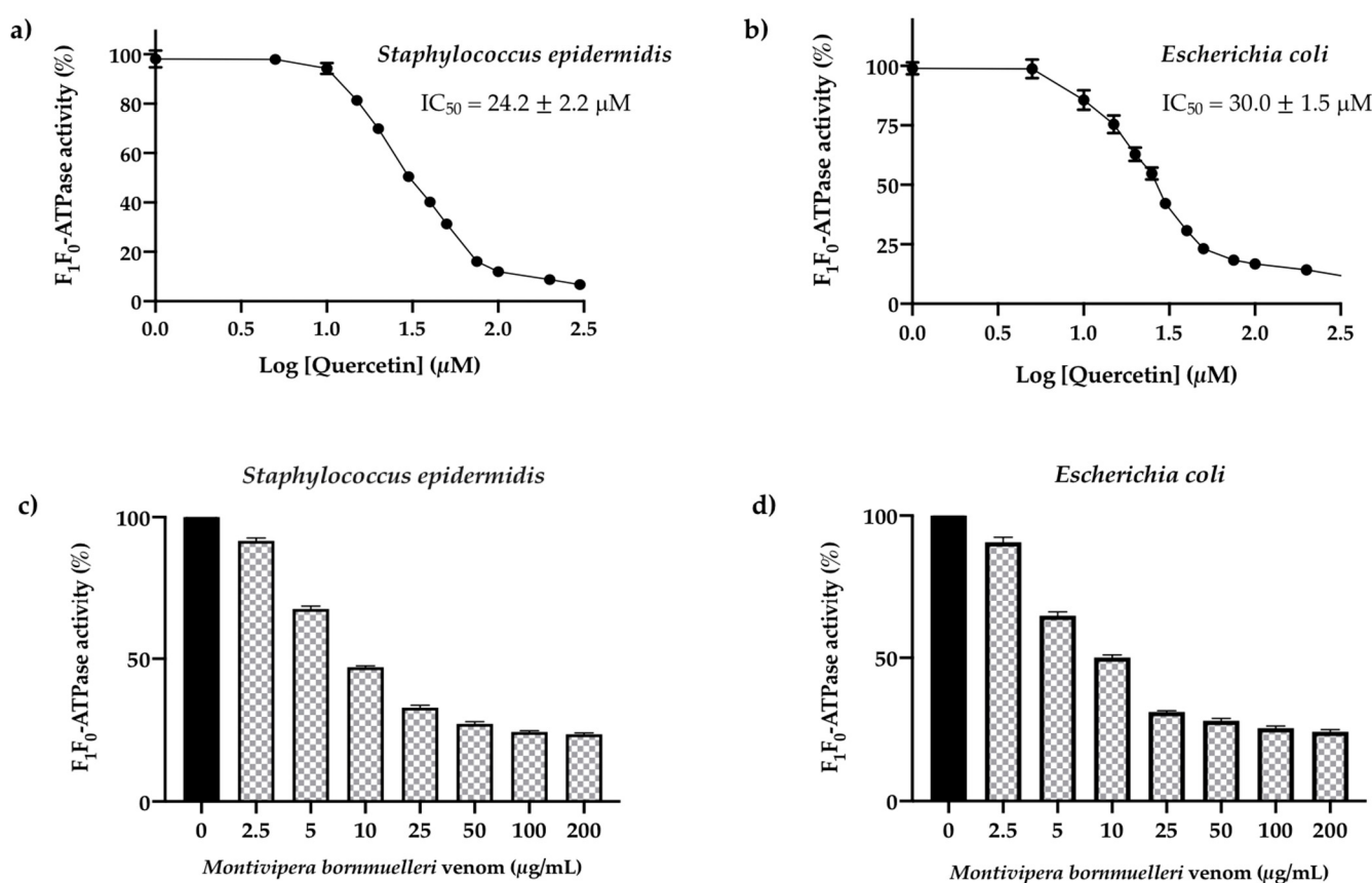
Figure 2. Effect of the M. bornmuelleri venom on the F_1F_0 -ATPase enzymatic activities of S. epidermidis and E. coli bacteria strains. The IC_{50} of the quercetin—used as an inhibitory reference ligand—on the enzymes is shown. (a) Dose-response curve showing the F_1F_0 -ATPase activity (%) of S. epidermidis as a function of the log of the concentration of quercetin. (b) Dose-response curve showing the F_1F_0 -ATPase activity (%) of E. coli as a function of the log of the concentration of quercetin. (c) Histogram representing the effect of M. bornmuelleri venom ( \mu g/mL ) on the activity (%) of membrane-bound S. epidermidis F_1F_0 -ATPase. (d) Histogram representing the effect of M. bornmuelleri venom ( \mu g/mL ) on the activity (%) of membrane-bound E. coli F_1F_0 -ATPase. For the four graphs represented here, the error bars show the standard deviation obtained from experiments carried out in triplicate. Data are expressed as mean \pm SD ( n = 3 ). Quercetin was used as a positive control. One-way ANOVA test: ns (not significant), when compared with the control. The M. bornmuelleri venom exerts a dose dependent inhibition on ATPase activity.
