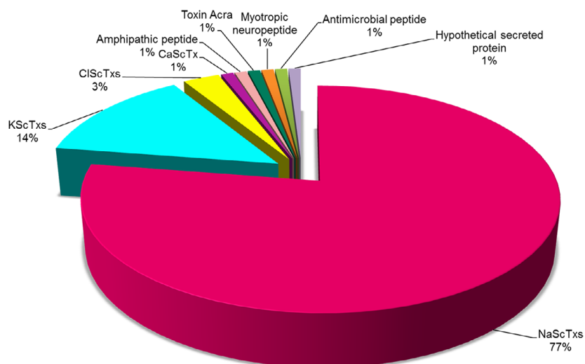
Fig. 6. Summary of the total peptides identified by top-down and bottom-up approaches. The 102 peptides were divided into neurotoxins, including NaScTx, KScTx, ClScTx, CaScTx and toxin Acra, amphipathic peptide, myotropic neuropeptide, AMPs, and hypothetical secreted protein.
