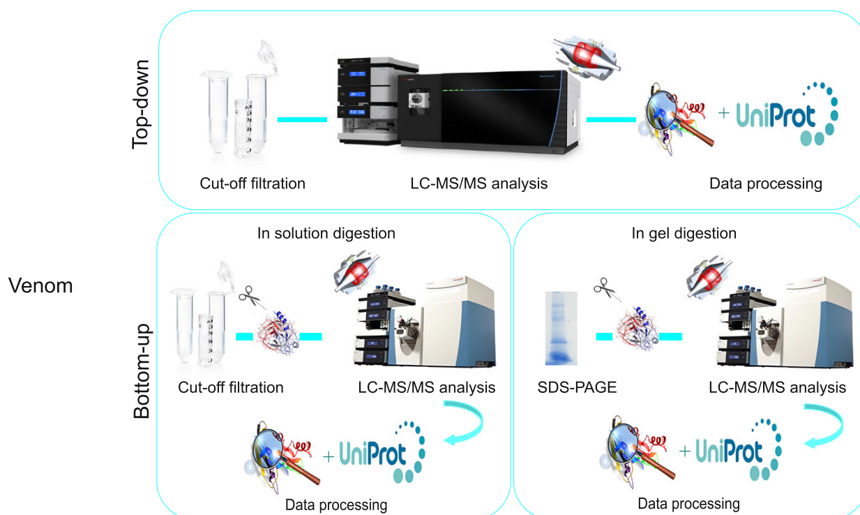
Fig. 1. Experimental workflow performed in this study. At first, B. occitanus venom was milked by electrical stimulation and applied to a 30 kDa filter. For the top-down venomics, the flow-through containing toxins < 30 kDa was analyzed by the Thermo Scientific™ Orbitrap Fusion Lumos Tribrid Mass Spectrometer. For the bottom-up approach, two digest methods were achieved: 1) in-solution digestion, the flow-through containing toxin < 30 kDa was directly reduced with DTT, alkylated with IAA, and digested with trypsin; and 2) in-gel digestion, the unstained gel was excised to small cubes, reduced, alkylated, and digested. The digest peptides were then desalted with ZipTip and applied to the Orbitrap Q-Exactive mass spectrometer.
