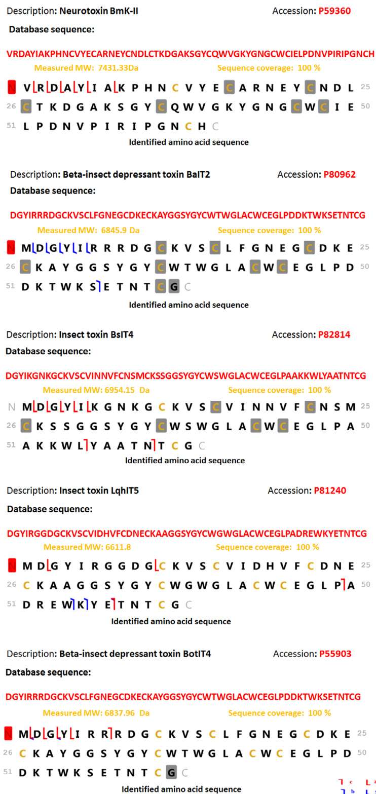
Fig. 4. The detected amino acid sequences of the five toxins identified with 100% coverage by the top-down LC-MS/MS; neurotoxin BmK-II (P59360); beta-insect depressant toxin BalT2 (P80962); insect toxin BslT4 (P82814); insect toxin LqhIT5 (P81240); and beta-insect depressant toxin BotIT4 (P55903).
