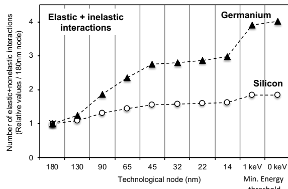
Figure 5. Relative evolution of the total number of elastic+inelastic interactions that produce a recoil nuclei satisfying the condition E > E_{min} . Values are normalized with respect to the ones corresponding to the 180 nm node.
