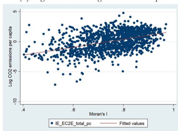
Fig. 2. Scatter plots across 1328 cities for the year 2015.
