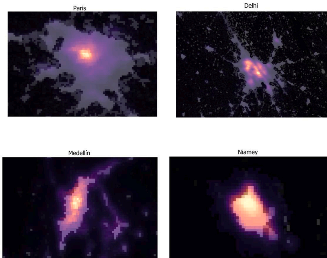
Fig. A.1. Spatial structure of four different cities.
