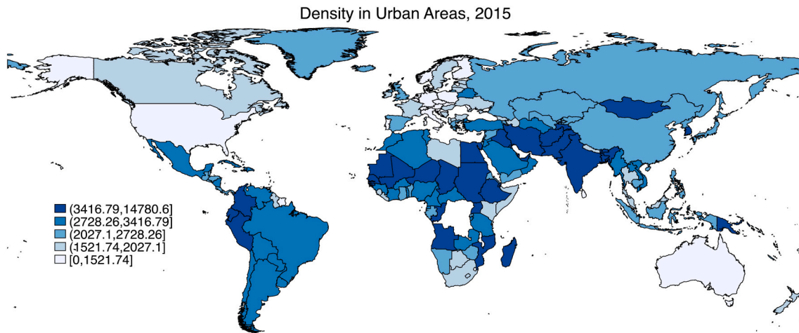
Fig. 3. Density in urban areas, 2015.
