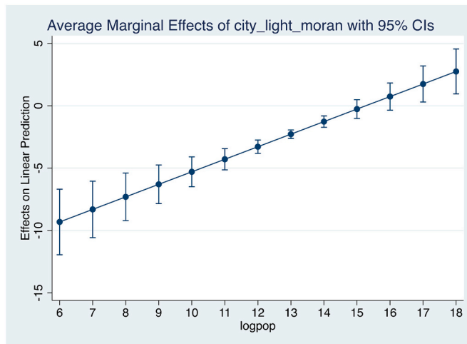
Fig. B.1. Marginal effects of structure depending on city size.
