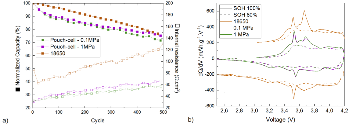
Figure 2: a) Normalized discharge capacity for cycles at C/5 and resistance (2C, 30s at 50% SOC) evolution upon cycling of 18650 cells at C and pouch cells at C/2 under constant pressure of 0.1 MPa and 1 MPa b) incremental capacity at state of health (SOH) of 100% (1 st post-formation cycle) and 80% (after 310 and 420 cycles for pouch and cylindrical cells, respectively) for various cells. SOH is defined as the capacity retention at C/5 in comparison to initial capacity at C/5. 18650 cell plots are shifted to +200 in charge and -200 mAh.g -1 .V -1 in discharge to ease reading the curves.
