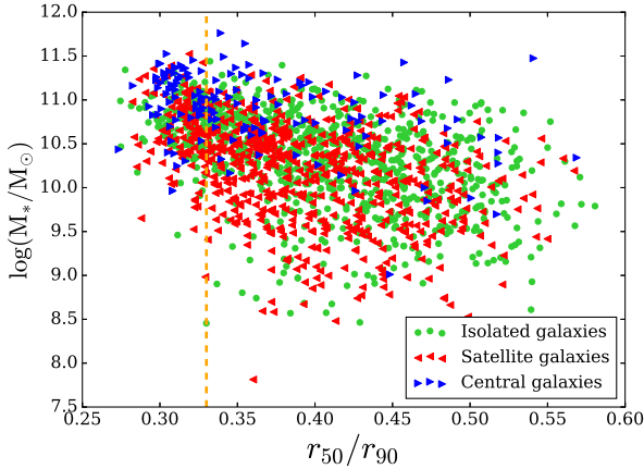
Figure 4. Same as Figure 2, but for the stellar mass vs. inverse concentration index distribution. The orange-dashed line shows the morphological selection we use (inverse concentration index r_{50}/r_{90} = 0.33 ).
