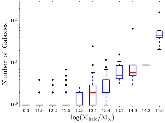
Figure 3. Box-and-whisker plot of number of galaxies in a halo of a certain mass. The width of halo mass bins is 0.3 in log scale. The red line indicates the mean number of galaxies in a halo and the box marks the first and third quartile of the data, while the whiskers mark the lowest and highest value still within 1.5 times the interquartile range. The outliers are marked as individual black dots. The figure shows that the median number of galaxies per halo increases with increasing halo mass and that the range in number of galaxies gets broader. Note that \log M_{\text{halo}} = 0 means that no mass was assigned to that halo.
