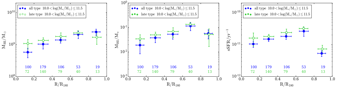
Figure 6. Averaged H I mass (left panel), H I mass fraction (middle panel) and specific star formation rate (right panel) for the all-type (blue filled points) and the late-type (green open points) satellites with stellar mass: 10^{10.0} < M_* \leq 10^{11.5} M_\odot , as a function of normalised projected group-centric radius. The error bars are estimated using jack-knife re-sampling. The numbers below the points show the number of galaxies in each radial bin. The corresponding values are presented in Table 1.
