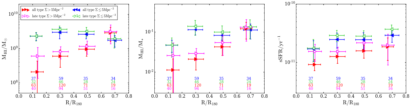
Figure 8. Same as Figure 6, with satellite galaxies in 10^{10.0} < M_* \leq 10^{11.5} M_\odot divided into two local density bins, above and below 5 \text{ Mpc}^{-2} (right-pointing and left-pointing triangles), respectively. The corresponding values are presented in Table 3.
