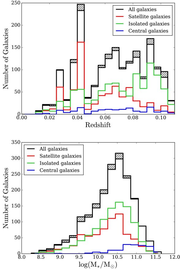
Figure 1. Redshift (top panel) and stellar mass (bottom panel) distribution for the SDSS spectroscopic sub-sample contained within the 35 WSRT pointings. The distributions for all galaxies, satellite galaxies, isolated and group central galaxies are shown by the black, red, green and blue lines, respectively. The hatched region shows the galaxies not included in Yang catalogue. The group catalogue is based on the main galaxy sample from SDSS DR7 and galaxies with a redshift completeness C \leq 0.7 are removed. The missing galaxies tend to be low-mass and faint. The interval for stellar mass bins and redshift bins are 0.2 dex and 0.005, respectively. The lower limit of the redshift of the selected sample is z = 0.01 , and the upper limit of the redshift is z = 0.11 . The average redshift of the sample is \langle z \rangle = 0.065 .
