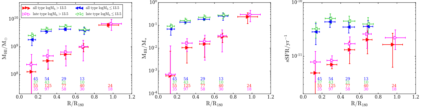
Figure 7. Same as Figure 6, with satellite galaxies in 10^{10.0} < M_* \leq 10^{11.5} M_\odot divided into two group halo mass bins, above and below 10^{13.5} h^{-1} M_\odot (right-pointing and left-pointing triangles), respectively. The results from the all-type and the late-type satellites are labeled as filled and open points, respectively. The corresponding values are presented in Table 2.
