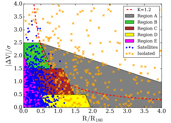
Figure 9. The phase-space diagram for the satellites (blue points) and isolated galaxies (orange crosses) in our sample. The red dashed line refers to the caustic profile with K = 1.2 . The colored five regions are given by Rhee et al. (2017), based on the time since infall.
