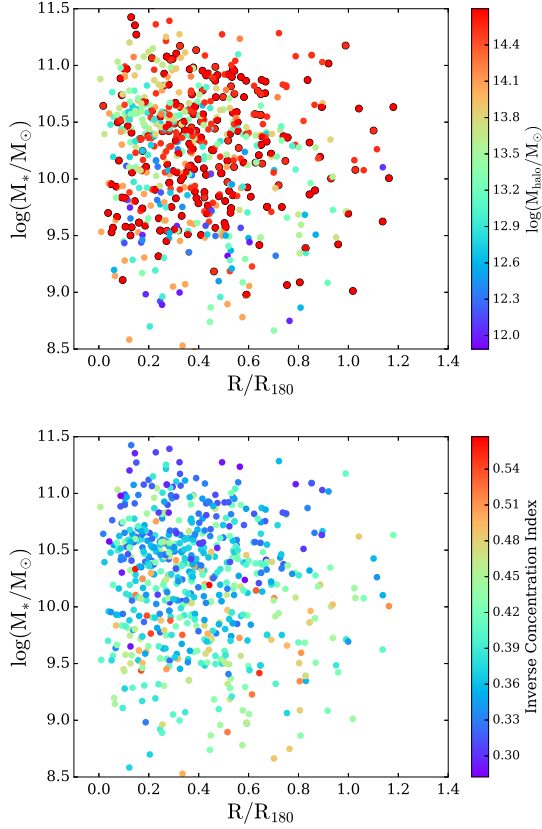
Figure 5. Stellar mass as a function of normalised projected group-centric radius for satellites, coloured according to the halo mass of the group the satellites are located in (upper panel) and their inverse concentration index (lower panel). The points with black circles refer to the satellites from the two largest groups.
