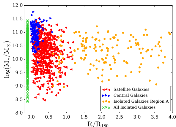
Figure 10. Stellar mass as a function of normalised projected group-centric radius for all galaxies in our sample. The centrals in groups, isolated galaxies and satellites are marked with blue right-triangles, green crosses and red left-triangles, respectively. Isolated galaxies are shifted from zero projected radius for clarity. The orange points are isolated galaxies located within Region A (see Figure 9) of a neighbouring group, and the group-centric radius is the distance to their nearest neighbouring groups.
