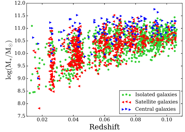
Figure 2. The stellar mass vs. redshift distribution for the SDSS spectroscopic sub-sample contained within the 35 WSRT pointings. The satellite, group centrals and isolated galaxies are shown by the red left triangles, blue right triangles and green points, respectively.
