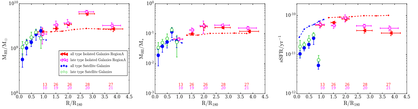
Figure 11. Same as Figure 6, but for satellite galaxies (circle points; see Fig. 6) and infalling isolated galaxies (left-pointing triangles) in the range 10^{10.0} < M_* \leq 10^{11.5} M_\odot as a function of normalised projected group-centric radius, extended out to greater radii. The results from the all-type and the late-type galaxies are labeled as filled and open points, respectively. For the isolated galaxies, the group-centric radius correspond to the distance from the galaxy to the centre of its nearest group. The corresponding values are presented in Table 4 and Table 1. Each panel also overplots the measurement from SHARK simulation with red and blue dashed line corresponding to the all-type satellite galaxies and infalling isolated galaxies.
