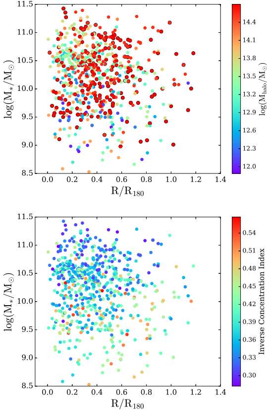
Figure 5. Stellar mass as a function of normalised projected group-centric radius for satellites, coloured according to the halo mass of the group the satellites are located in (upper panel) and their inverse concentration index (lower panel). The points with black circles refer to the satellites from the two largest groups.
