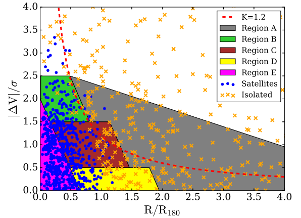
Figure 9. The phase-space diagram for the satellites (blue points) and isolated galaxies (orange crosses) in our sample. The red dashed line refers to the caustic profile with K = 1.2 . The colored five regions are given by Rhee et al. (2017), based on the time since infall.
