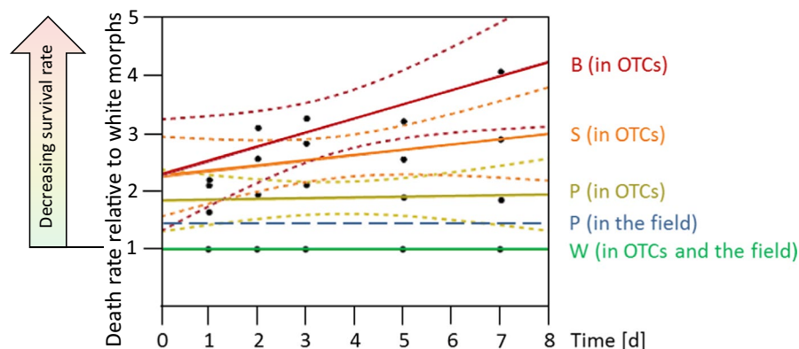
FIGURE 5 Mortality of naturally and artificially pigmented T. pisana morphs in the field population and the global warming-simulating experiment at Montfavet, Southern France, relative to the white morph (green, set to 1.0). The mortality of naturally pigmented (P) individuals in the natural situation is 148% of that of whites (blue dashed linear regression line). In case of experimental warming in open-top chambers of 1.12^{\circ}\text{C} on the average, the mortality rate of P morphs increases by a factor of 1.26%–187% of the whites, on the average (yellow-green, linear regression with 95% confidence intervals). The mortality rates in artificially striped (S, orange line) and blackened (B, red line) individuals increased with time of exposure to simulated global warming and showed that these morphs would not persist under these conditions
