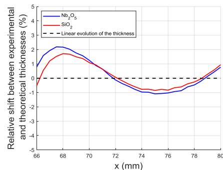
Fig. 4. Relative shift between the experimental and theoretical thickness gradient for single layers of SiO 2 and Nb 2 O 5 in the linear gradient region (right).
