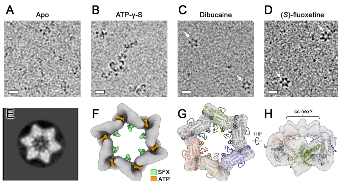
Figure 5. SFX and dibucaine stabilize the 2C hexamer. (A) Cryo-electron micrographs of apo, (B) ATP- \gamma -S incubated, (C) dibucaine incubated or (D) SFX incubated hex \Delta 116-2C (scale bar = 10 nm). (E) Representative 2D class average from untilted micrographs of SFX incubated hex \Delta 116-2C. Weak density can be observed within the central of the 2C hexamer. (F) Surface representation of the 12 Å resolution cryo-EM map of hex \Delta 116-2C in complex with SFX, generated from 30° tilted cryo-EM data. The map is shown at a contour level of 0.0661 and the binding positions of SFX (green) and ATP (orange) are superposed. (G) As shown in (F) with a hexameric 2C model, generated using the crystal structure of the monomer, overlaid. For clarity, pore-loop residues 85-100 are omitted. (H) A 110° rotated view of the model shown in (G), with the map shown at a contour level of 0.059. Putative density for the linker and cc-hex is indicated.
