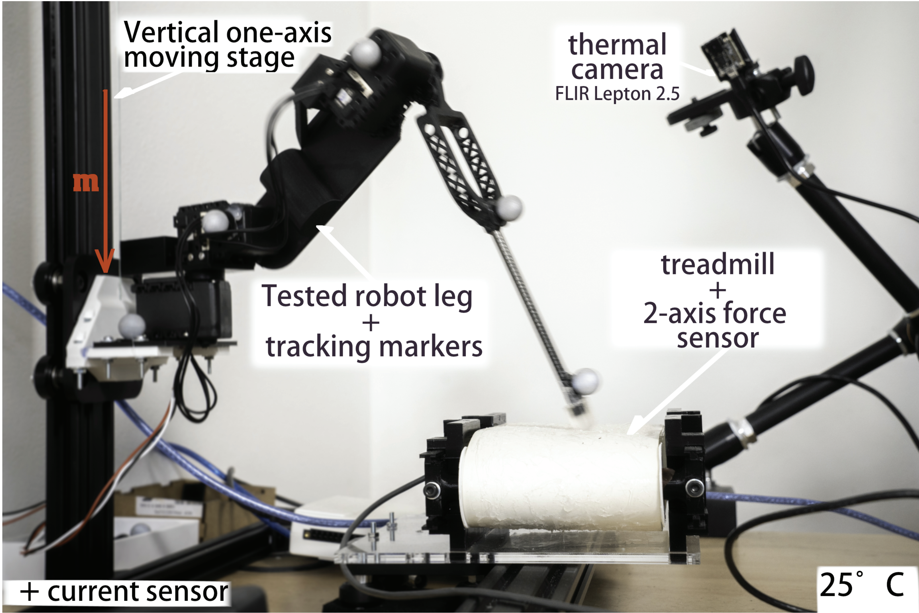
Leg test bench photography. ©Tifenn Ripoll - VOST Collectif / Institut Carnot STAR (2021)
