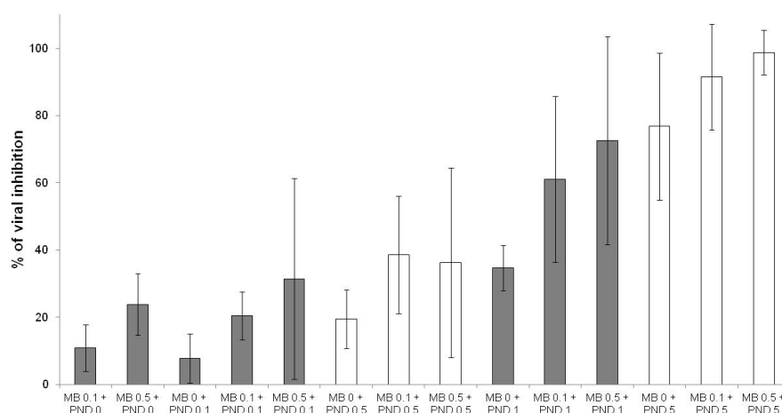
Figure 5. Antiviral activities of methylene blue (MB) at 0.1 and 0.5 \mu\text{M} in combination with pyronaridine (PND) at 0.1, 0.5, 1 and 5 \mu\text{M} (error bars represent standard deviation of 9 independent experiments).
