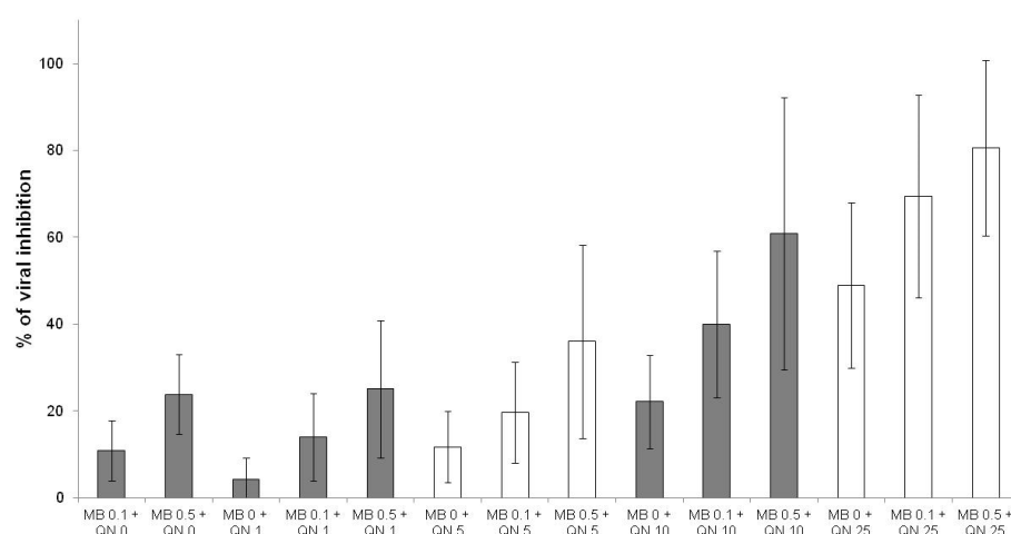
Figure 3. Antiviral activities of methylene blue (MB) at 0.1 and 0.5 \mu\text{M} in combination with quinine (QN) at 1, 5, 10 and 25 \mu\text{M} (error bars represent standard deviation of 13 independent experiments).
