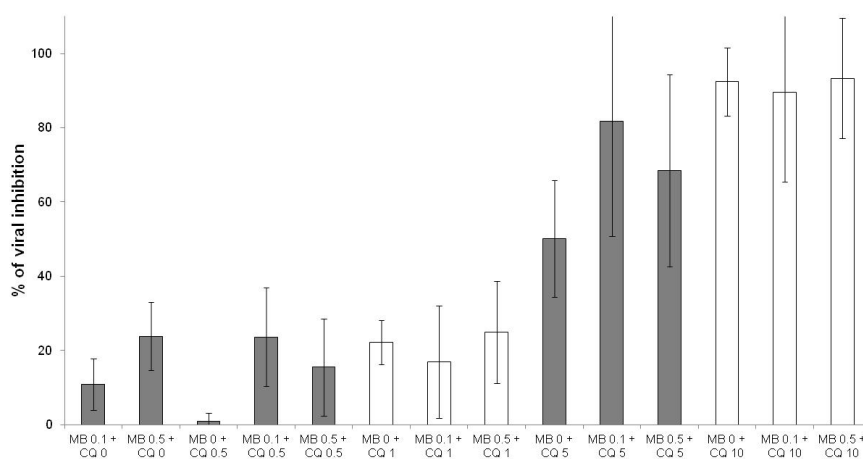
Figure 6. Antiviral activities of methylene blue (MB) at 0.1 and 0.5 \mu\text{M} in combination with chloroquine (CQ) at 0.5, 1, 5 and 10 \mu\text{M} (error bars represent standard deviation of 9 independent experiments).
