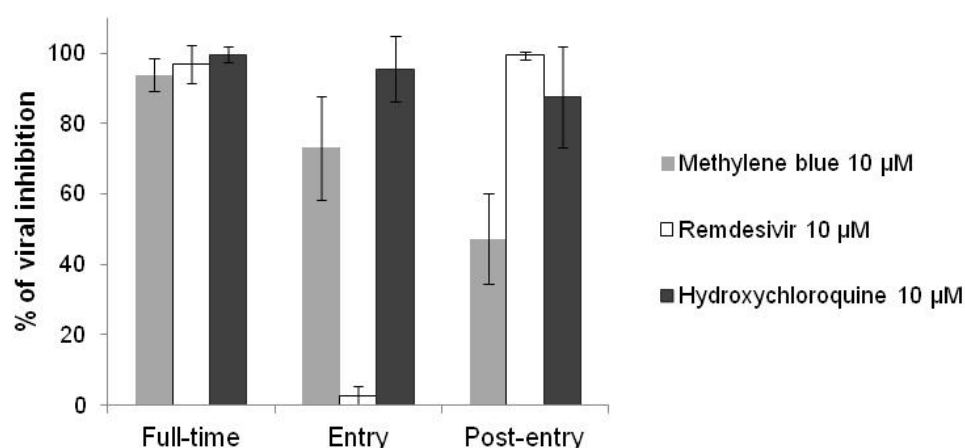
Figure 2. Antiviral activities of methylene blue, hydroxychloroquine and remdesivir at 10 \mu\text{M} against the SARS-CoV-2 IHUMI-3 strain in vitro. For “full-time” treatment, Vero E6 cells were infected with the IHUMI-3 strain for 48 h after pre-incubation of the cells with one of the three drugs for 4 h. For “entry” treatment, the cells were infected for 2 h after pre-incubation for 4 h and then the virus–drug mixture was replaced with fresh medium maintained for 46 h. For “post-entry” treatment, the cells were infected for 2 h and then incubated with drug for 46 h. Error bars represent standard deviation of 6 to 9 independent experiments.
