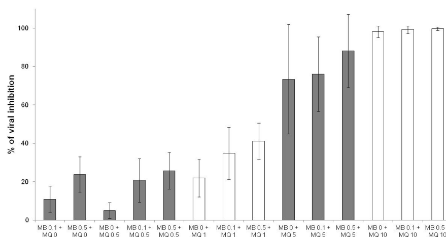
Figure 4. Antiviral activities of methylene blue (MB) at 0.1 and 0.5 \mu\text{M} in combination with mefloquine (MQ) at 0.5, 1, 5 and 10 \mu\text{M} (error bars represent standard deviation of 13 independent experiments).
