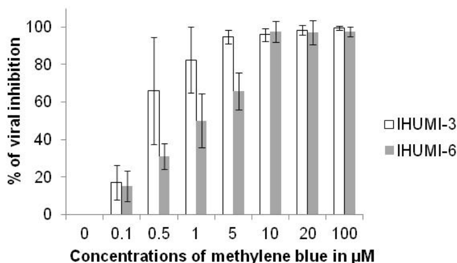
Figure 1. Anti-SARS-CoV-2 activity of methylene blue in % of antiviral inhibition on IHUMI-3 (mean of 12 independent experiments) and IHUMI-6 (mean of 6 independent experiments) clinically-isolated strains (error bar represents standard deviation).
