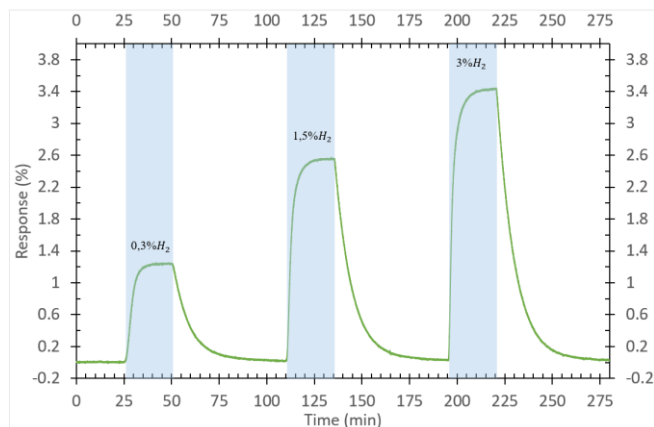
Figure 8. Sensor responses to 0.3%, 1.5% and 3% H_2 in N_2 at 50°C.
