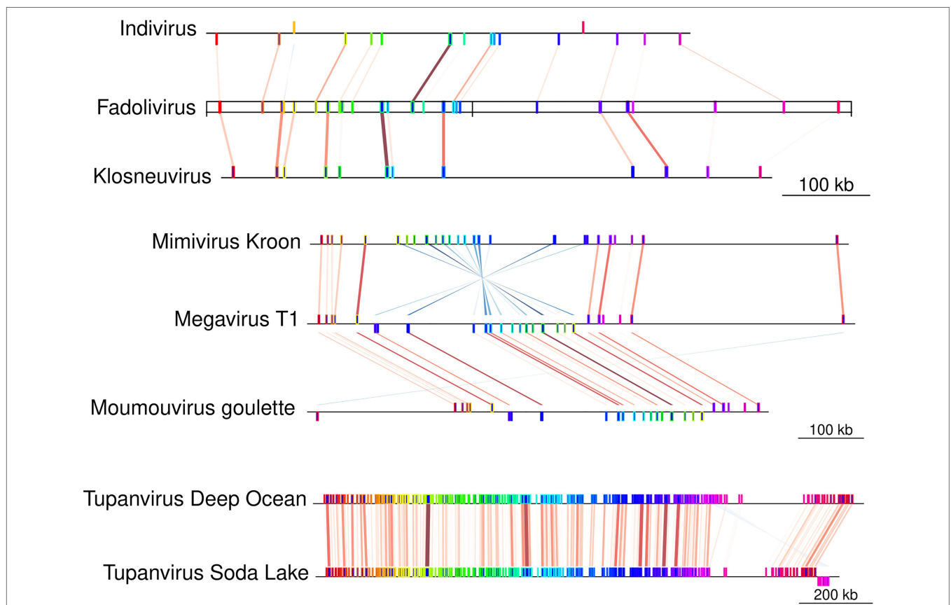
FIGURE 3 | Block synteny comparison between Fadolivirus and other Klosneuvirinae genomes. Conserved genomic regions (Mauve conserved blocks) between Fadolivirus and its closest relatives, Klosneuvirus and Indivirus. Contigs in Indivirus and Klosneuvirus have been reordered based on the Fadolivirus genome. For comparison, conserved regions are also shown between selected members of the proposed subfamily Megamimivirinae, including Tupanviruses.
