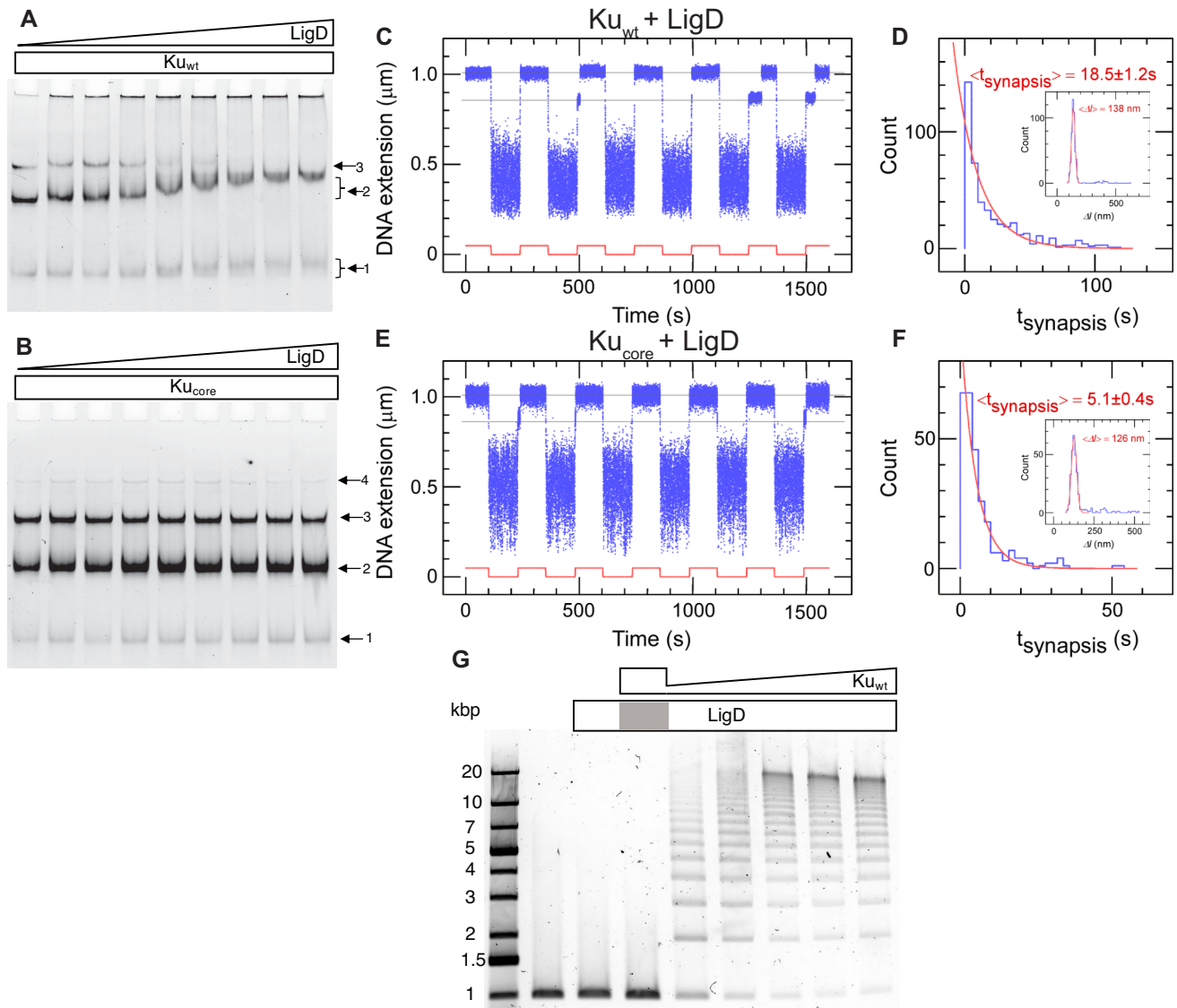
Figure 3. The C-terminal arms of Ku are required for recruitment of LigD and full stabilization of the pre-ligation complex. EMSA gel of a 50 bp blunt-ended DNA substrate incubated with 0.2 \mu M (A) Ku_{wt} and (B) Ku_{core} and an increasing concentration of LigD (0–0.8 \mu M , 0.1 \mu M increments). The arrows indicate the number of Ku homodimers loaded on the DNA substrate. (C) Time-trace of molecular forceps experiment (blue), where a blunt-ended DNA substrate is used together with Ku_{wt} (5 nM) and LigD (5 nM). End-to-end synapses were detected upon repeated force cycling (red). (D) Lifetime distribution of the specific end-binding events is fit to a single-exponential, giving a mean lifetime of 18.5 \pm 1.2 s (SEM, n = 459 ). End-specific events are identified (inset) as having a \Delta l value within three standard deviations of the mean expected amplitude change given bridge mechanics (Gaussian fit in red, \langle \Delta l \rangle = 138 \pm 15 nm, SD, n = 486 ). (E, F) as C and D but for Ku_{core} , giving a mean synapsis lifetime of 5.1 \pm 0.4 s (SEM, n = 270 ). End-specific events are identified (inset) as having a \Delta l value within 3 standard deviations of the mean expected amplitude change given bridge mechanics (Gaussian fit in red, \langle \Delta l \rangle = 126 \pm 16 nm, SD, n = 305 ). (G) Ligation of a 1000 bp blunt-ended DNA substrate with a constant amount of LigD (0.1 \mu M ) and increasing concentration of Ku_{wt} (0–1 \mu M , 0.2 \mu M increments). The grey area in the LigD bar indicates the absence of LigD in the corresponding sample, where only Ku is added at a concentration of 1 \mu M .
