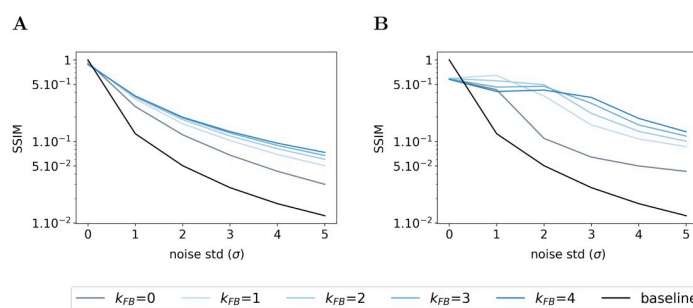
Fig 11. Effect of the feedback strength on noisy images from face database. This figure description is similar to the description of the Fig 10B and 10C. For the face database, all presented curves represent the median structural similarity index over 400 samples of the testing set.
