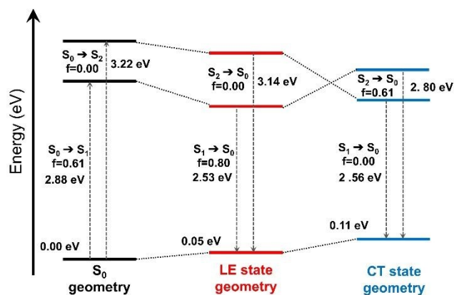
Figure 5. Evolution of the ground-state and excited-state energies, and of oscillator strengths with respect to different optimized geometries of the ground-state ( S_0 ) and the excited-states (LE and CT states) of B-4 . The interaction type and MOs involved in these transitions are shown in Figure S16.
