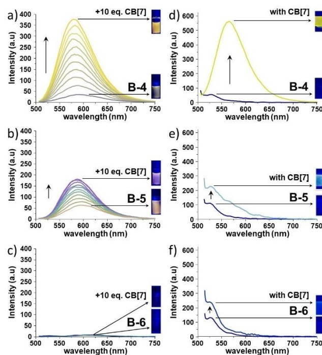
Figure 1. Fluorescence spectra of (a) B-4 , (b) B-5 , and (c) B-6 ( 1.0 \times 10^{-5} M each, excitation wavelength = 490 nm) in water upon addition of CB[7] and solid state fluorescence spectra of (d) B-4 , (e) B-5 , and (f) B-6 without and with CB[7].
