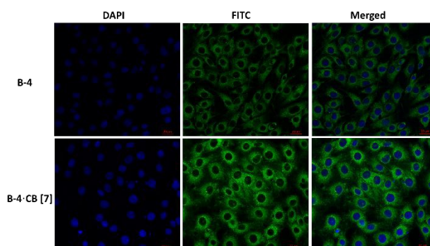
Figure 7. Confocal fluorescence microscopy images of U87 cells after incubation with B-4 without (top line), and with (bottom line) CB[7] for 4 hours. Cell nuclei were stained with DAPI after PFA fixation (DAPI, \lambda_{\text{Ex/Em}} = 405/450 nm; FITC, \lambda_{\text{Ex/Em}} = 488/520 nm).
