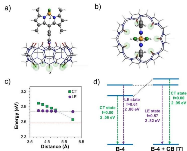
Figure 6. Different views (a, b) of the minimized B-4 •CB[7] complex. The B-4 –CB[7] distance is plotted in c) against the energy of the CT and LE states in the optimized CT geometry of B-4 . The red and blue dotted lines represent the energies of CT and LE states respectively for isolated B-4 (the distance between CB[7] and B-4 is from the guest carbon atom of the methyl-pyridinium and from the barycenter of the host oxygen atoms; green circles). Energy diagram in d) illustrating how the energy of the excited-state is impacted by CB[7] complexation and corresponding to a host-guest distance of 4.25 Å (lowest energy structure for the B-4 •CB[7] complex).
