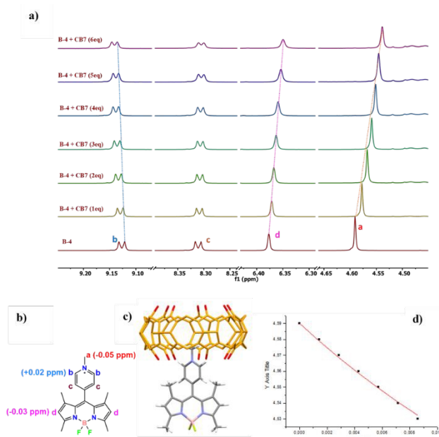
Figure 3. a) ^1\text{H} -NMR titration of B-4 (0.5 mM) with CB[7] in \text{D}_2\text{O}/\text{CD}_3\text{CN} (80:20) solution, b) assignment of the corresponding protons chemical shifts and c) Lowest energy DFT minimized structure of the 1:1 inclusion complex of B-4 + CB[7] d) The chemical shift of guest molecule Ha versus CB[7] concentration and the non-linear curve fit in red.
