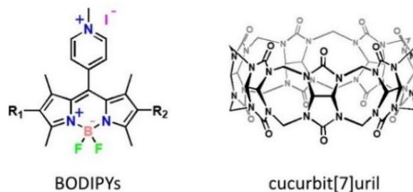
Chart 1. Structures of BODIPYs and CB[7] used in this work (R1, R2 = H or I).
