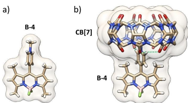
Figure 4. X-ray structure of B-4 and DFT minimized structure of the B-4 •CB[7] complex (hydrogen bonds: dashed lines, hydrogens of CB[7] removed for clarity).
