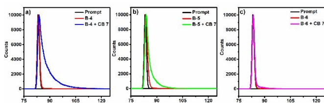
Figure 2. Fluorescence decay profiles of a) B-4 without and with CB[7], b) B-5 without and with CB[7], and c) B-6 (10 \times 5 M) without and with CB[7] using laser excitation at 390 nm.
