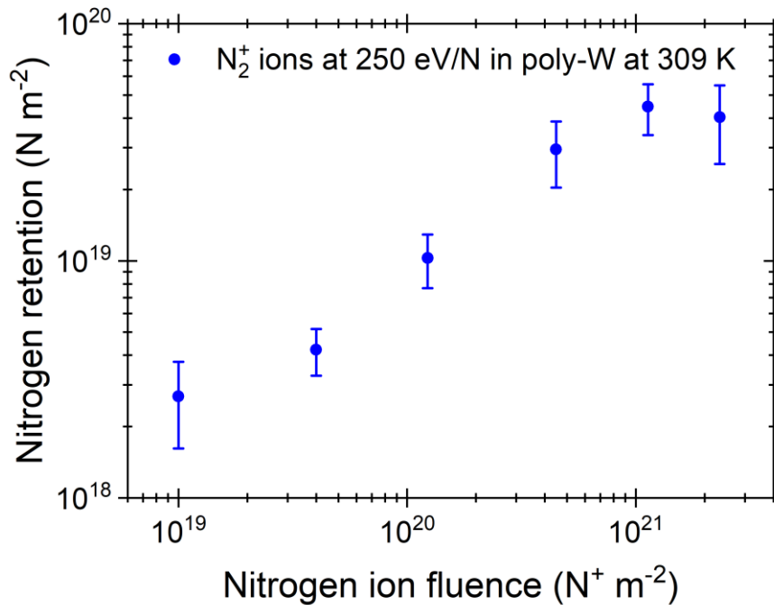
Figure 1. Evolution of the nitrogen retention in tungsten as a function of nitrogen ion fluence.
