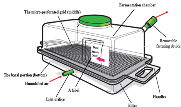
FIGURE 1 Schematic representation of Zymotis-2 bioreactor
