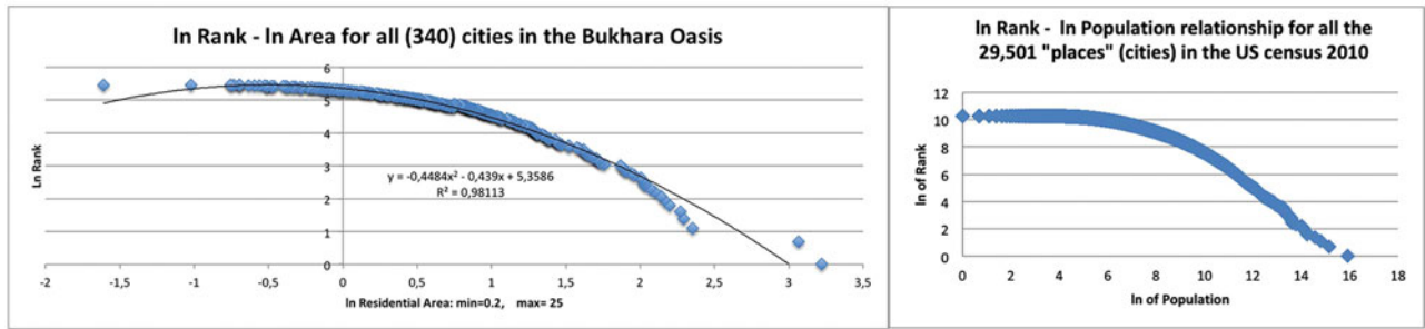
Figure 7. Rank size distribution: Bukhara oasis (left) and USA (right).
