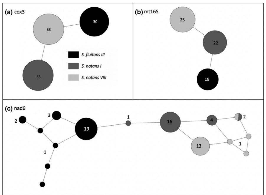
FIGURE 2 Haplotype networks for (a) cox3 gene, (b) mt16S rRNA gene, and (c) nad6 gene. Each node (circle) represents a distinct haplotype (nucleotide sequence) and is scaled to the number of samples with that particular sequence. The numbers within and adjacent to each node reflect sample size. Each line represents a single-nucleotide difference between nodes. Grayscale indicates the pelagic Sargassum morphotype from which the sequence was generated
