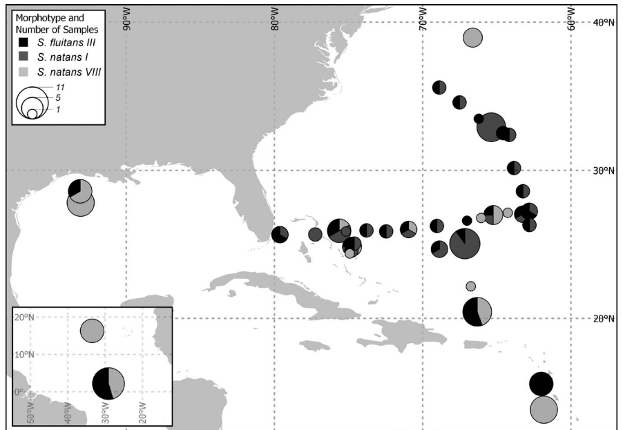
FIGURE 1 Distribution of pelagic Sargassum samples, collected from 2015 to 2019 during Sea Education Association cruises, as well as from the Gulf of Mexico and equatorial Atlantic expeditions
