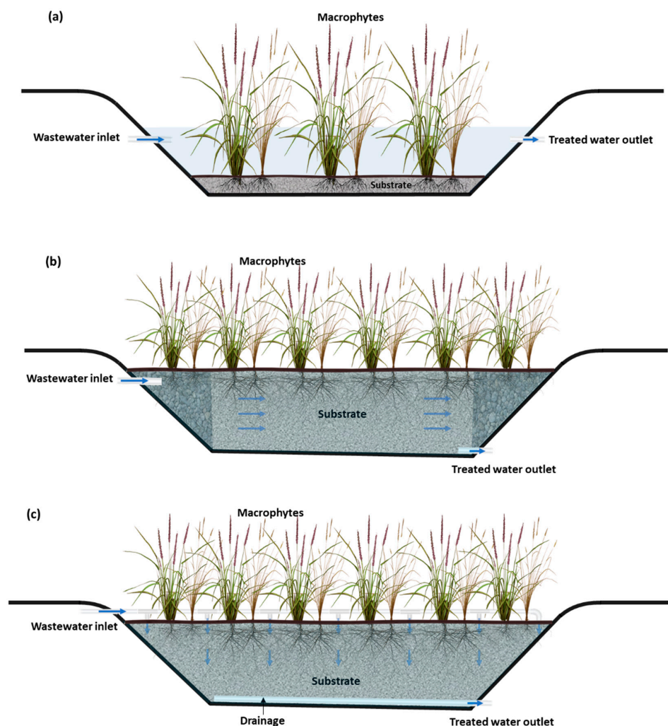
Figure 1. Free water surface CW (a); horizontal subsurface flow CW (b); vertical subsurface flow CW (c).
