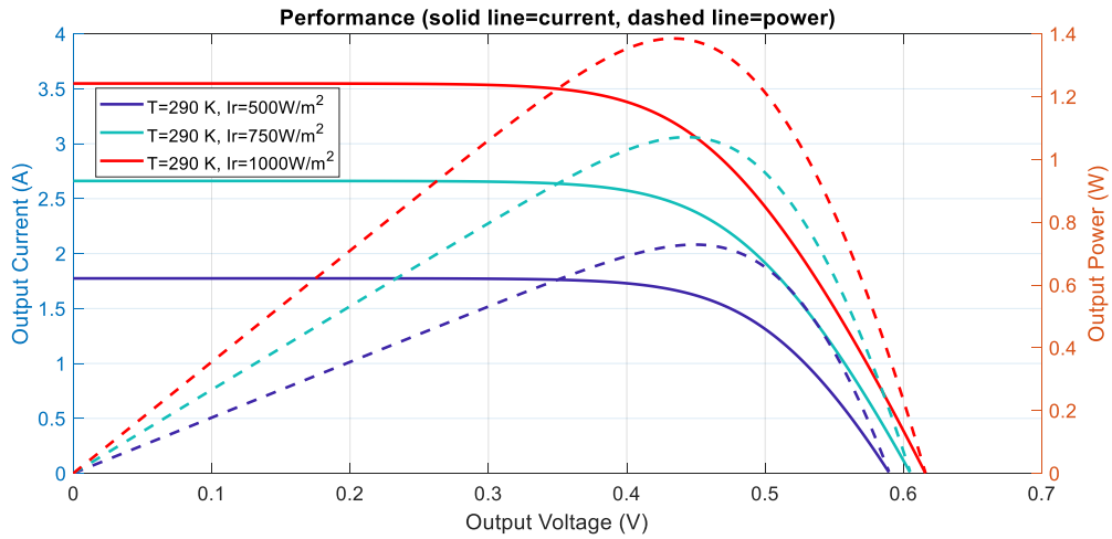
Figure 9: Evolution of the cell performance according to the variation of effective irradiance ( 500\text{ W/m}^2 , 750\text{ W/m}^2 and 1000\text{ W/m}^2 ). The ambient temperature and exposed surface are considered constant: 290^\circ\text{ K} for the ambient temperature and 0.01\text{ m}^2 for the surface.
