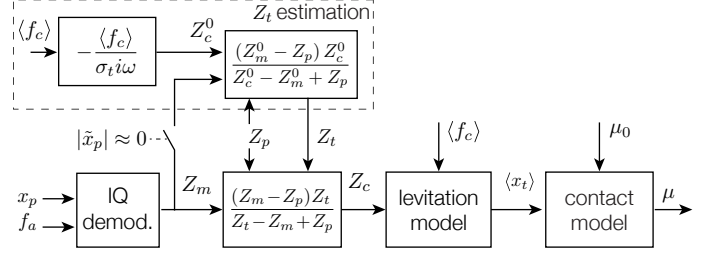
Fig. 12. The impedance Z_m is recovered from the IQ demodulation. The fingertip impedance Z_t is assumed to be constant during each trial and is found from the impedance at initial contact Z_c^0 . Meanwhile, the contact stiffness for every vibration amplitude is recovered from its impedance estimation, Z_c . The interfacial gap \langle x_t \rangle is then estimated from Z_c and \langle f_c \rangle . Lastly, the friction coefficient is estimated from Persson's model and initialized with the measured friction coefficient without vibration.
