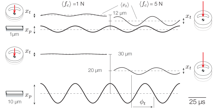
Fig. 8. Time-domain vibration of the plate and fingertip for two forces (1 N left and 5 N right) and two amplitudes (1 μm top row and 10 μm bottom row). The vibration of the skin decreases for the larger amplitude while the average height due to levitation increases.
