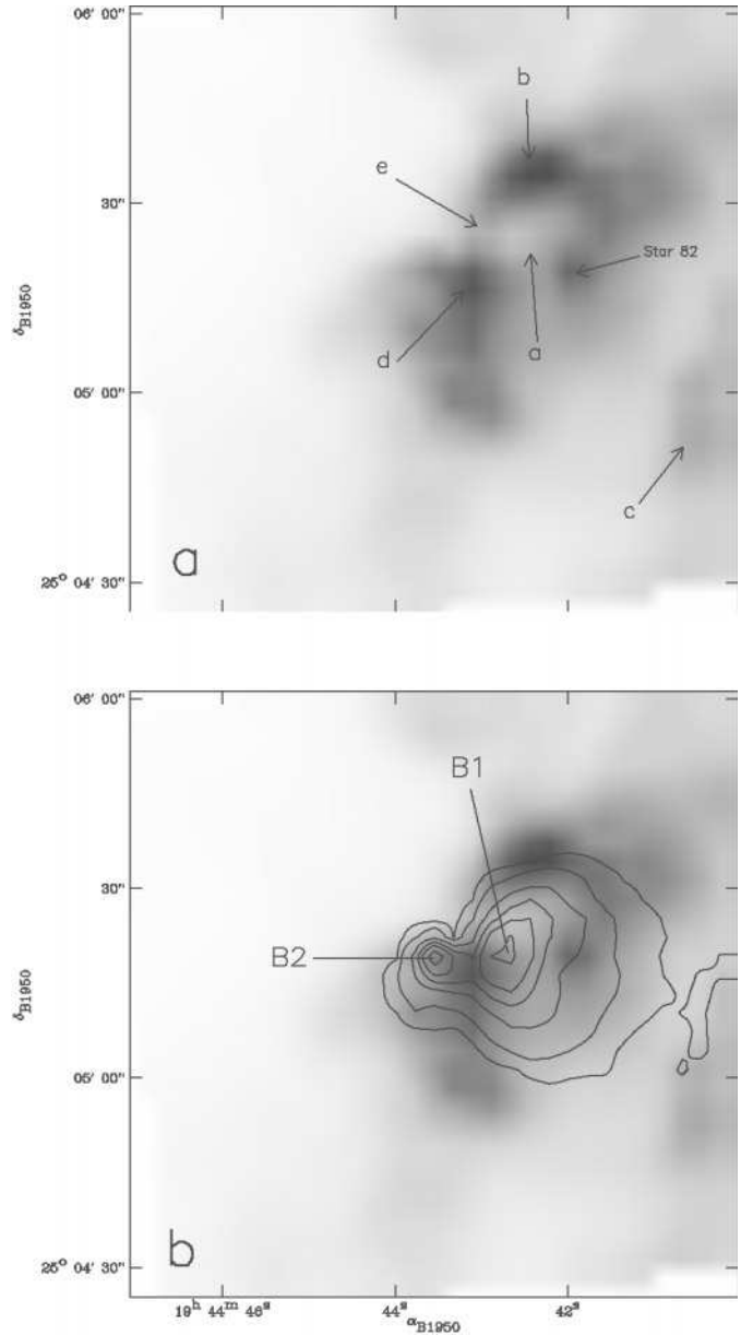
Fig. 7. a LW2 ( 5\text{--}8.5\ \mu\text{m} ) emission of the Sh2-88B region observed with ISOCAM. Star 82 and the zones discussed in the text are identified. b VLA map of 6\ \text{cm} emission, superimposed on the LW2 emission.
