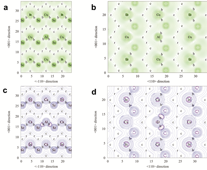
Fig. 7 Electron density (top panels) and Laplacian (bottom panels) distribution of CuIn 0.75 Al 0.25 Se 2 in plane (110) (a) (c) and plane (-110) (b) (d). b, c, and r mean bond, cage, and ring critical points. Green lines represent the electron density \rho , magenta and blue lines represent the negative and positive \nabla^2\rho , respectively.
