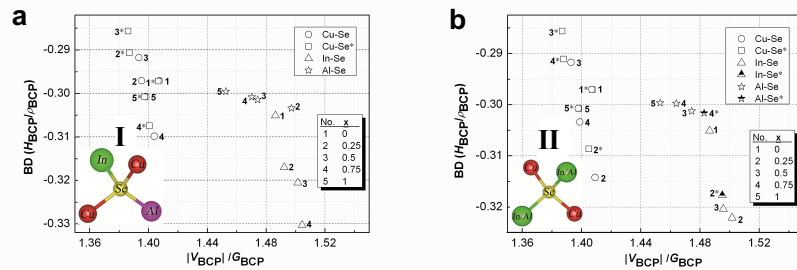
Fig. 9 Values of bond degree ( BD=H_{BCP}/\rho_{BCP} ) vs. |V_{BCP}|/G_{BCP} at BCPs of M-Se as x varies from 0 to 1. Structures I (Cu/In/Al-Se, a) and II (Cu/In-Se or Cu/Al-Se, b) represent two different constitutive parts of every unit cell. The asterisk sign (*) stands for the longest bond length for each pairwise M-Se.
