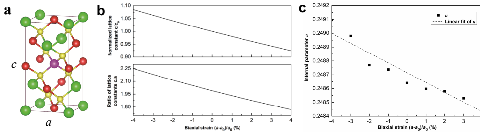
Fig. 10 Geometric characteristics of \text{CuIn}_{0.75}\text{Al}_{0.25}\text{Se}_2 and their evolution under biaxial strains (a-a_0)/a_0 . Unit cell (a), green, red, yellow and magenta atoms represent In, Cu, Se and Al, respectively. lattice constant ratio c/c_0 and c/a (b) and internal parameters u(\text{Se}) (c).
