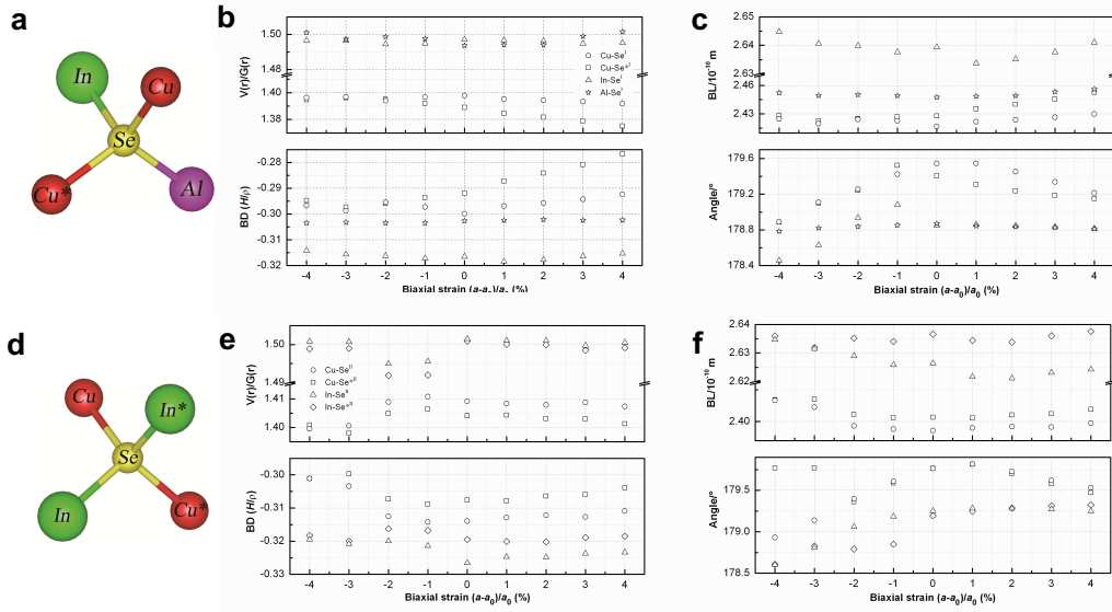
Fig. 13 Topological properties at bond critical points of structure I (a) and structure II (d) vs. biaxial strain ( a-a_0/a_0(\%) ). (b) and (e): ratio of potential energy density to kinetic energy density |V_{CP}|/G_{CP} and bond degree BD; (c) and (f): bond length BL and bond angle.
