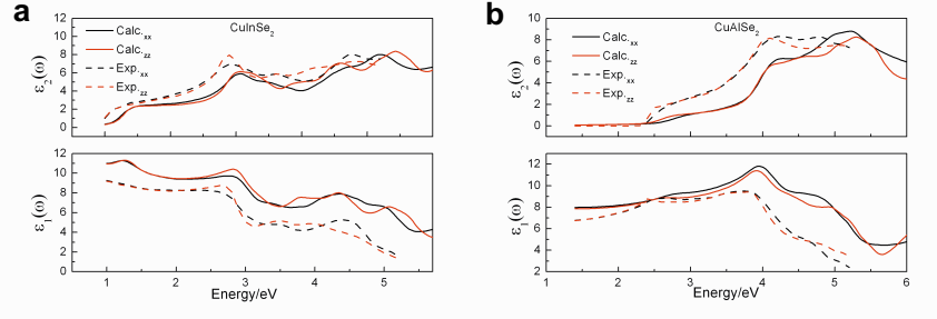
Fig. 5 Calculated (solid lines) and experimental (dash lines) results of dielectric functions of CuInSe 2 (a) and CuAlSe 2 (b) in the perpendicular ( xx , black lines) and parallel ( zz , red lines) directions to c -axis. The experimental data are taken from Ref. 39,40 .
