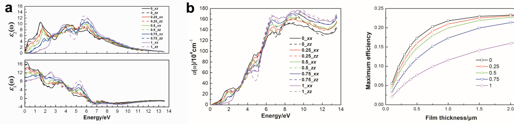
Fig. 6 Dielectric functions (a) and absorption coefficient (b) for CuIn 1-x Al x Se 2 at different x values. The solid lines and dashed lines represent the perpendicular ( xx ) and parallel ( zz ) directions to c -axis, respectively. Calculated maximum efficiency (c) with respect to the film thickness in the energetic domain [1.5;3.1] eV.
