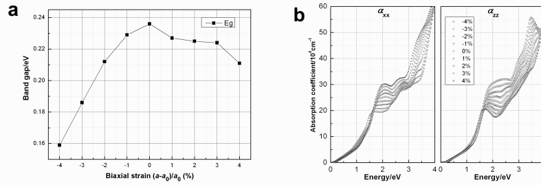
Fig. 11 Band gap vs. biaxial strain( a-a_0 )/ a_0 (%) (a) and absorption coefficient in perpendicular ( xx ) and parallel ( zz ) directions to c -axis vs. incident energy for various biaxial strains ( a-a_0 )/ a_0 (%) (b).
